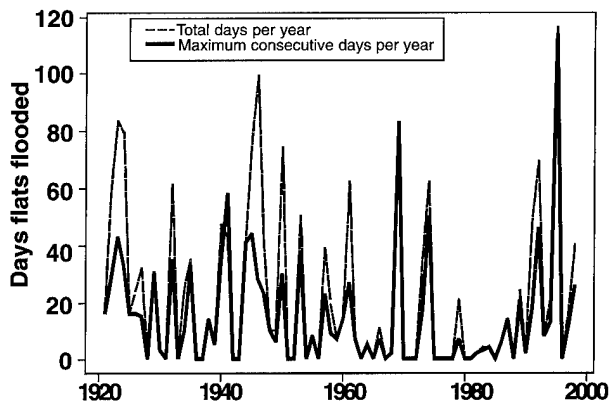
Figure 5-1. Total and maximum consecutive days flooded for the flats at the wet study site, 1920-90.
