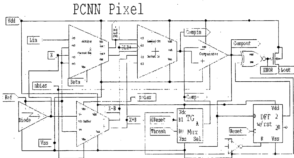
Figure 5. Optical Input PCNN Chip.
