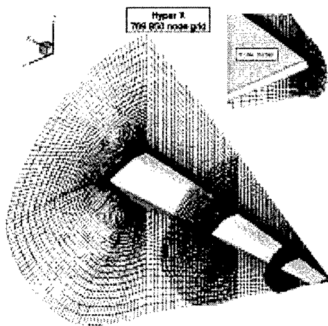
Figure 6 : Hyper-X mesh
