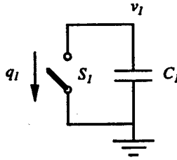
Figure 5: Computing the Energy Dissipated in a Switch
