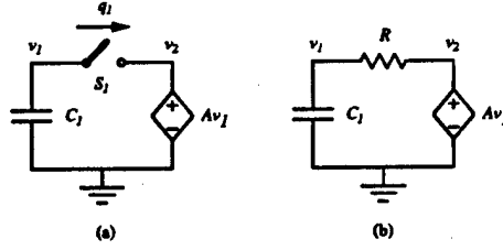
Figure 8: Negative Energy Dissipation in a Switch
