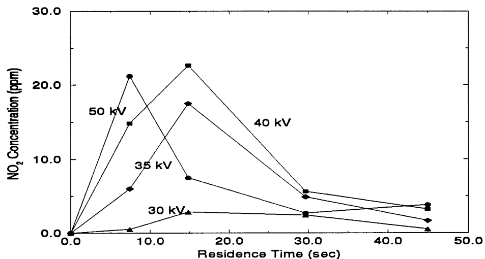
Figure 5.18: \text{NO}_2 Concentration Profile in an Atmosphere of Humid Air
