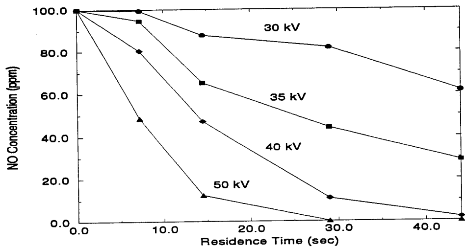
Figure 5.5: NO Concentration Profile in an Atmosphere of Nitrogen
