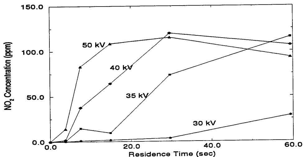
Figure 5.11: NO 2 Concentration Profile in an Atmosphere of Dry Air
