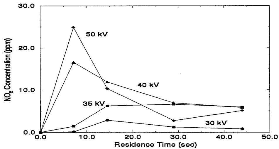
Figure 5.24: NO 2 Concentration Profile in an Atmosphere of Humid Air and CO
