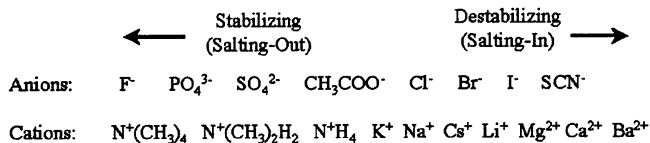
Figure 1. The Hofmeister (lyotropic) series of inorganic ions. Anions and cations are ranked in the order (from left to right) of their increasing destabilizing effects on proteins. The ions that are the most stabilizing tend to promote "salting-out" of proteins (Hochachka and Somero, 1984; Yancey, 1994).
