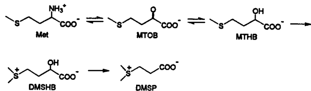
Figure 1. The biosynthesis of DMSP from Met in marine algae. In vivo isotope tracer data indicate that the first two steps are reversible (Gage et al., 1997).
