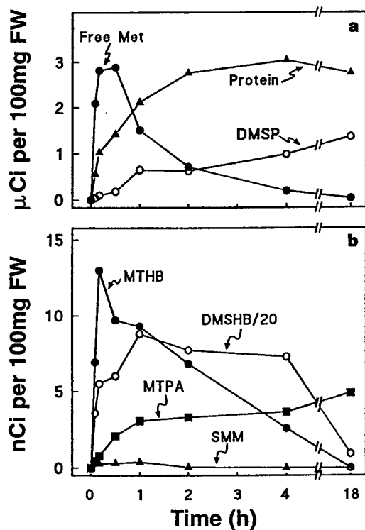
Figure 1 Labelling kinetics of selected small molecules and protein following administration of a tracer [ 35 S]Met dose to E. intestinalis . Batches of fronds (100 mg fresh weight, FW) were supplied with 5 \mu\text{Ci} (0.5 nmol) [ 35 S]Met. a , Free Met, DMSP and protein; b , Potential DMSP pathway intermediates; DMSHB data points are reduced by a factor of 20; MTPA, 3-methylthiopropylamine. No label ( \leq 0.5 nCi per 100 mg) was detected in 3-dimethylsulphoniopropionaldehyde.
