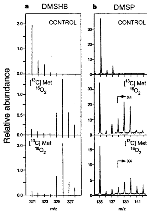
Figure 2 Evidence for conversion of DMSHB to DMSP by an oxygenase reaction in E. intestinalis . Fronds (100 mg) were incubated for 24 h with L-[U- 13 C 6 ]Met (5 \mu\text{mol} ) in flasks initially containing 21% 16 O 2 or 18 O 2 in N 2 ; controls received no Met and no 18 O 2 . a , SIM analysis of DMSHB. The peak areas in the control fit the expectation for natural-abundance C, S, Si and O isotopes. In the [ 13 C]Met/ 16 O 2 treatment, endogenous DMSHB was replaced by 13 C 4 - and 13 C 5 -labelled species (the S -demethylated derivatives of [ 13 C 6 ]- and [ 13 C 5 ]DMSHB). Exposure to 18 O did not change this pattern, showing that the \alpha -hydroxyl group does not originate from O 2 . b , FAB-MS analysis of DMSP. In the [ 13 C]Met/ 16 O 2 treatment, the peaks at m/z 139 and 140 are [ 13 C 4 ]- and [ 13 C 5 ]DMSP. Under 18 O 2 , the signals at m/z 141 and 142 ([ 13 C 4 , 18 O]- and [ 13 C 5 , 18 O]DMSP) show that 30–40% of the 13 C-labelled DMSP molecules contain an 18 O atom.
