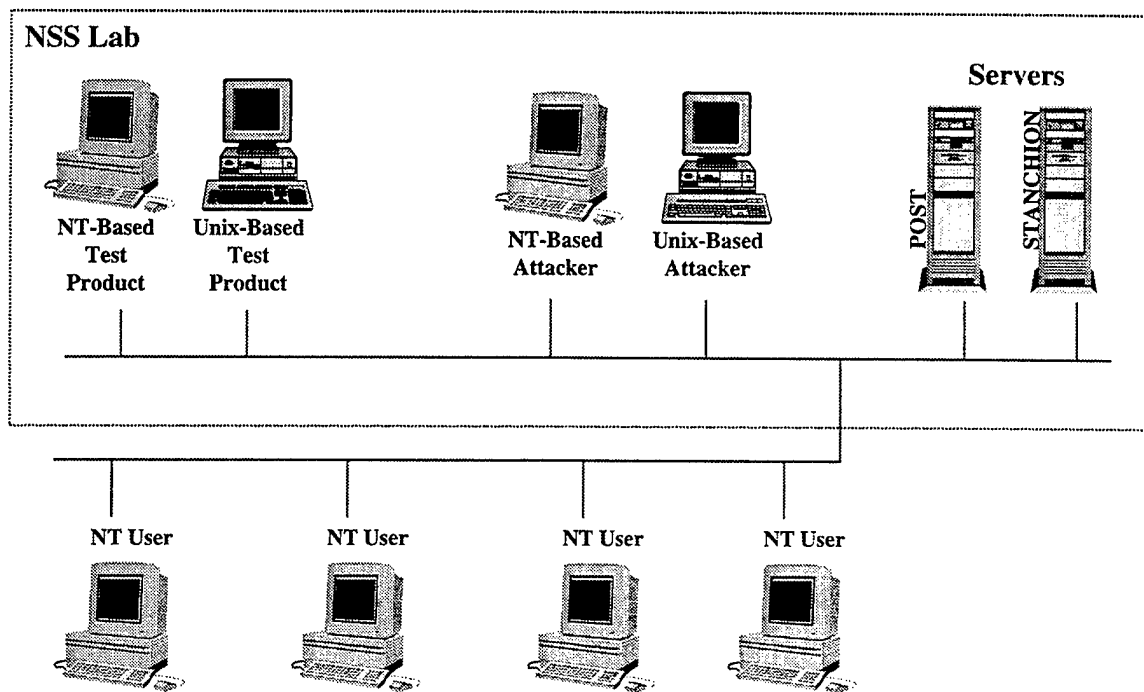
Figure 10. Generic test configuration.
