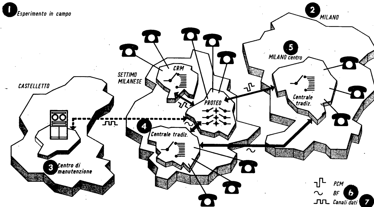
Figure 10. Introduction of the peripheral exchange in the Settimo Milanese network.
