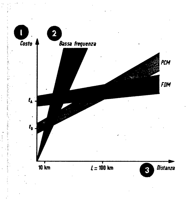
Figure 1. Transmission costs (per channel). Key: 1. cost; 2. low frequency; 3. distance
