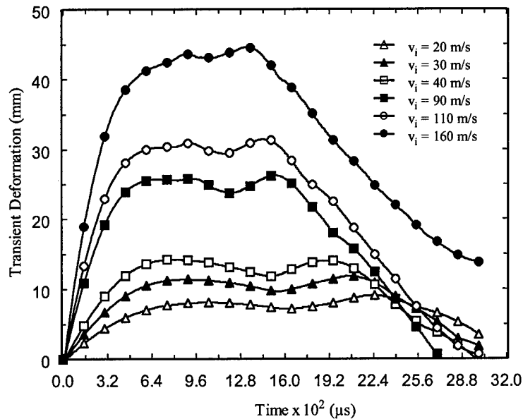
FIGURE 9 –Target's back plane transient deformation as a function of time for six different impact velocities ranging from 20 to 160 m/s
