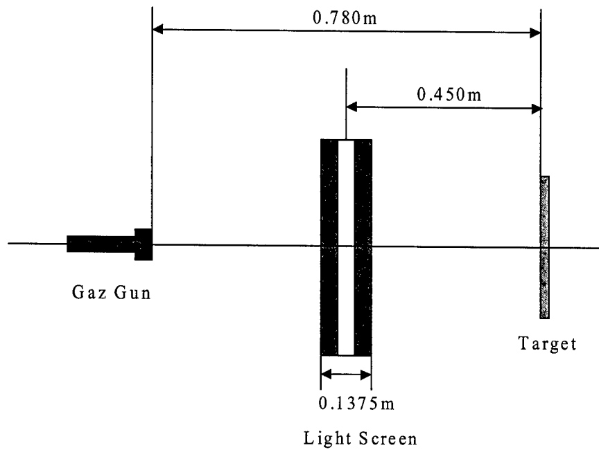
FIGURE 3 - Relative distance used in test set-up
