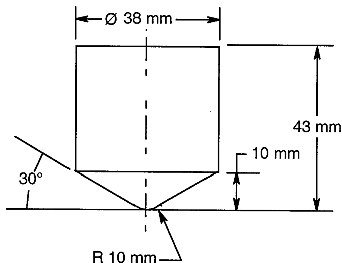
FIGURE 6 - Schematic drawing of the polycarbonate fragment simulating projectile
