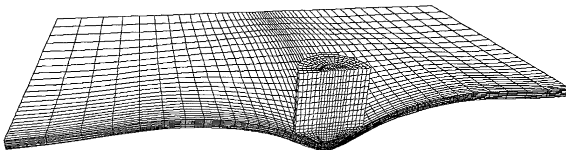
FIGURE 8 - Typical simulation performed to investigate the backplane deformation of a polycarbonate plate struck by a polycarbonate projectile
