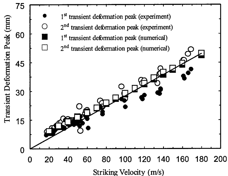
FIGURE 10 - Comparison of numerical and experimental transient deformation of the backface of the target plate
