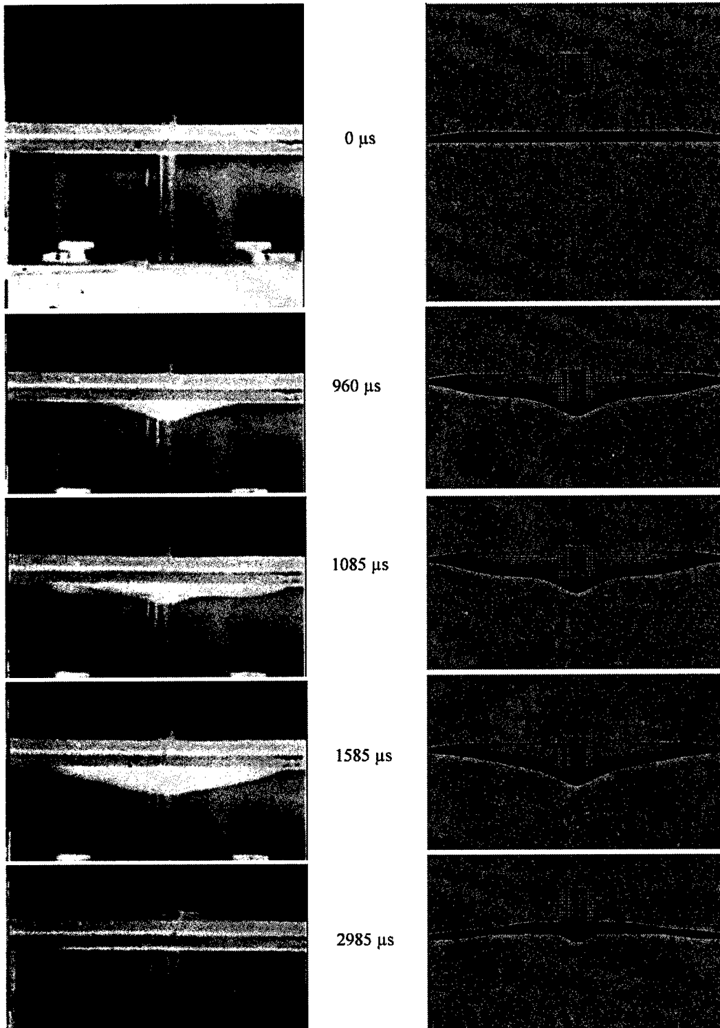
FIGURE 11 - Experimental and numerical comparison of target's backplane transient deformation. Projectile impact velocity is 118 m/s.
