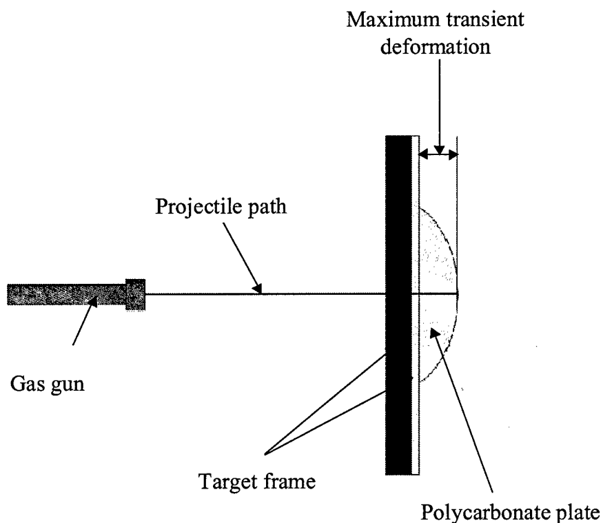
FIGURE 5 – Schematic diagram showing maximum transient deformation measurement
