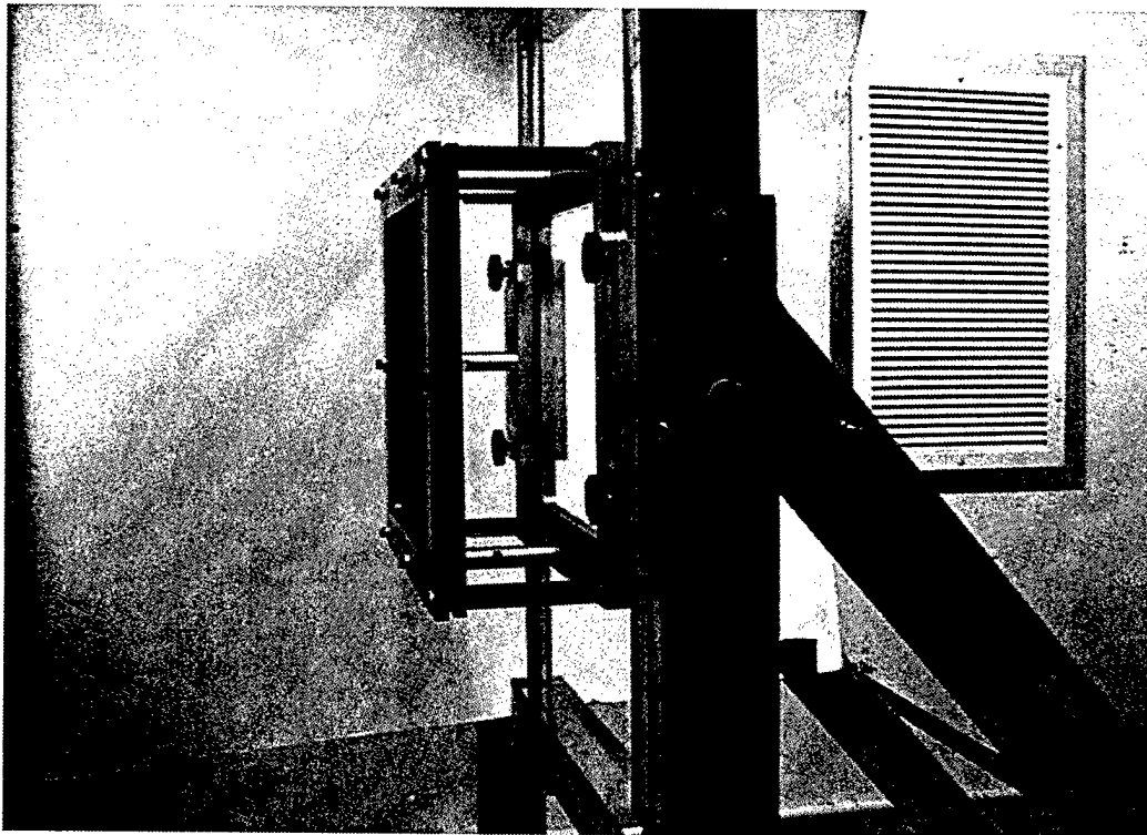
FIGURE 4 - Close up view of target frame fixture
