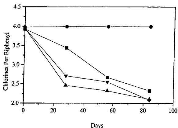
FIG. 3. Dechlorination rates of Baltimore Harbor cultures treated with physiological inhibitors. Symbols: ▲, no inhibitor; ■, 3 mM BES; ●, 20 mM sodium molybdate; ▼, 100-µg/ml vancomycin.
