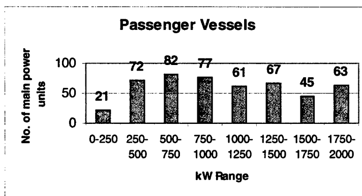
Figure 17. Passenger Vessel Main Power Unit kW Breakdown
