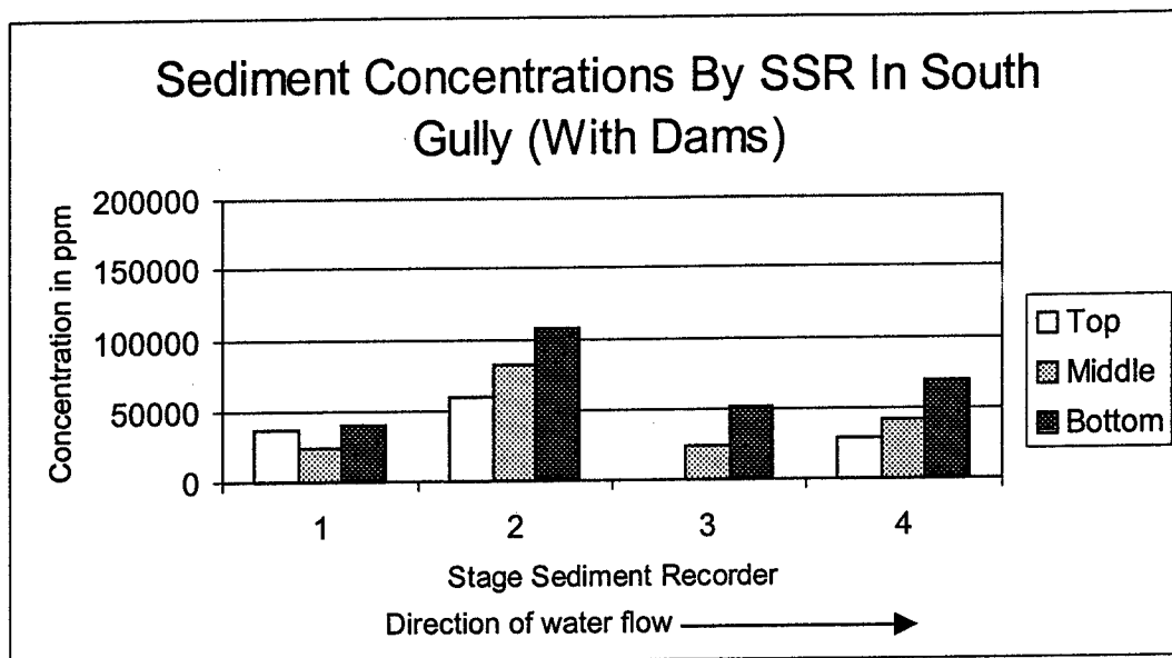
Figure 17. Suspended sediment concentrations from SSRs 1 – 4 in the south gully.
