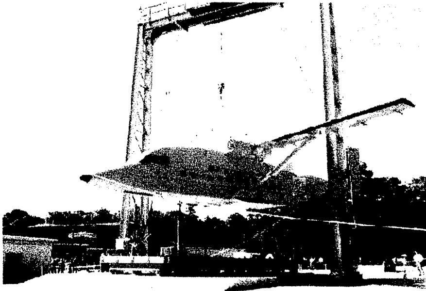
FIGURE 21. OVERALL PRETEST
