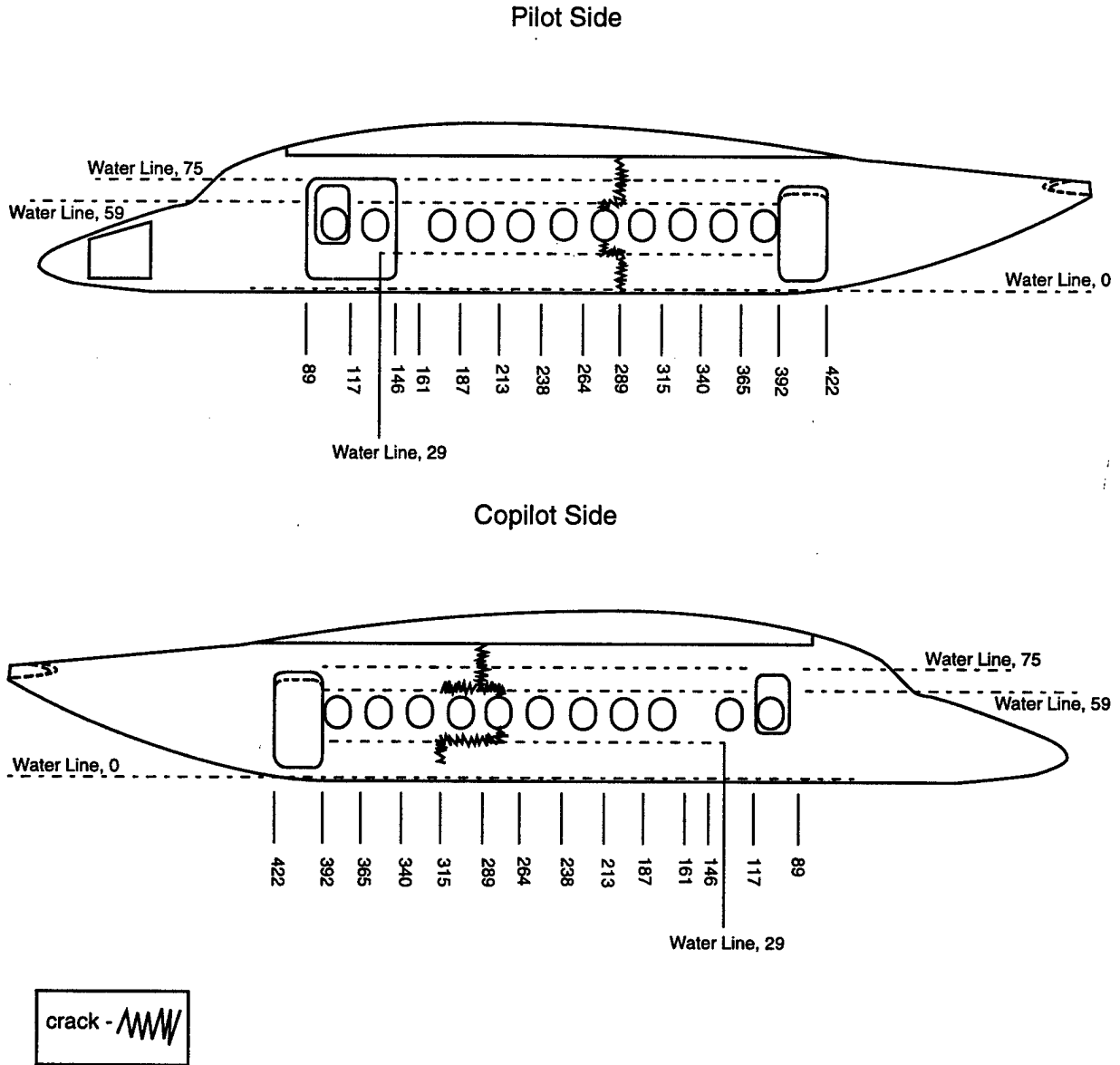
FIGURE 11. FUSELAGE CRACK
