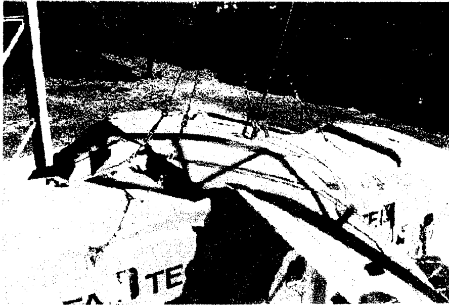
FIGURE 25. EXTERIOR FUEL TANK DEFORMATION POSTTEST
