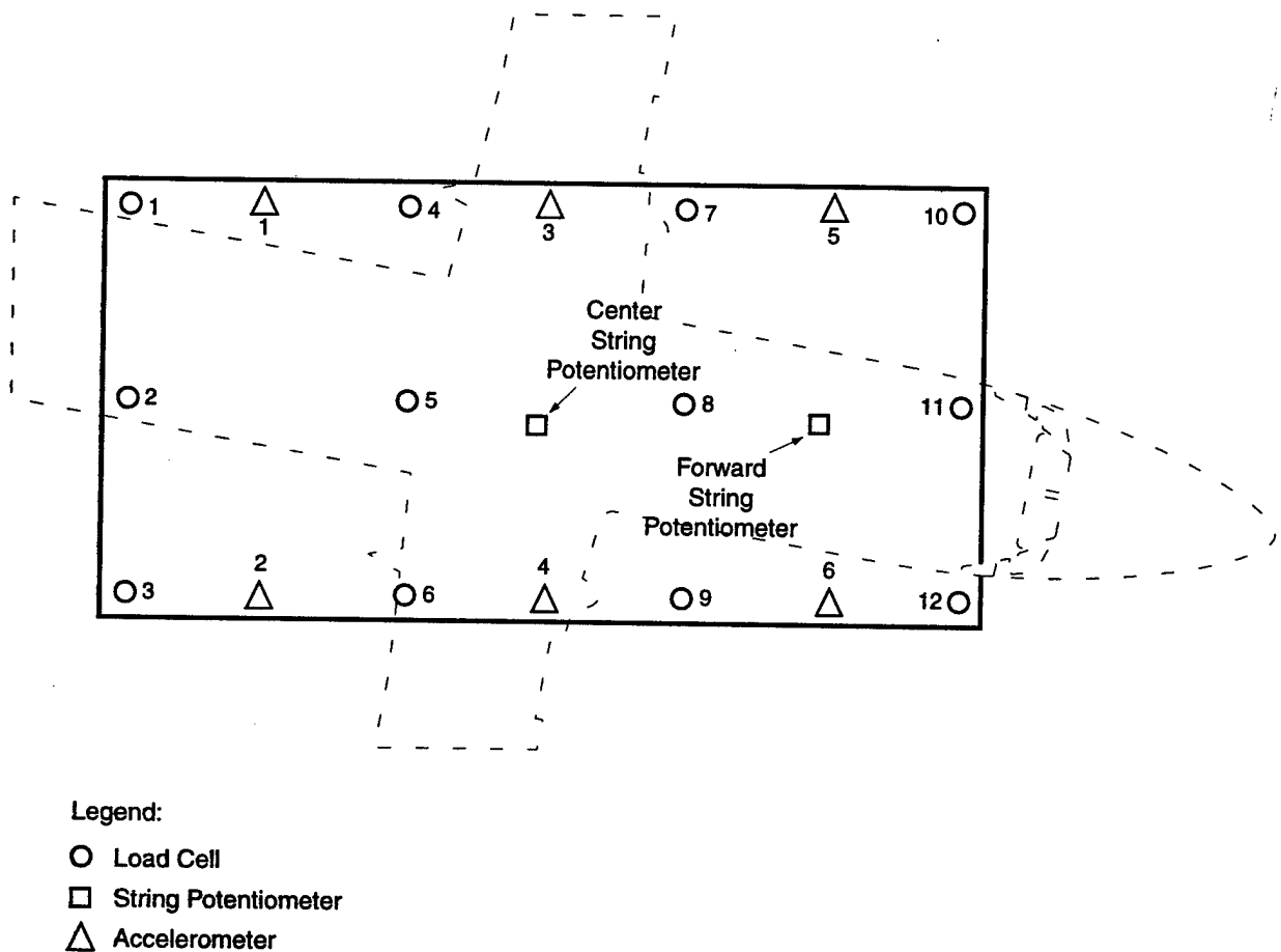
FIGURE 5. PLATFORM INSTRUMENTATION
