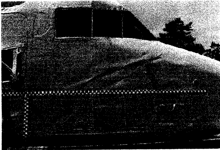
FIGURE 24. SKIN BUCKLING COPILOT-SIDE POSTTEST
