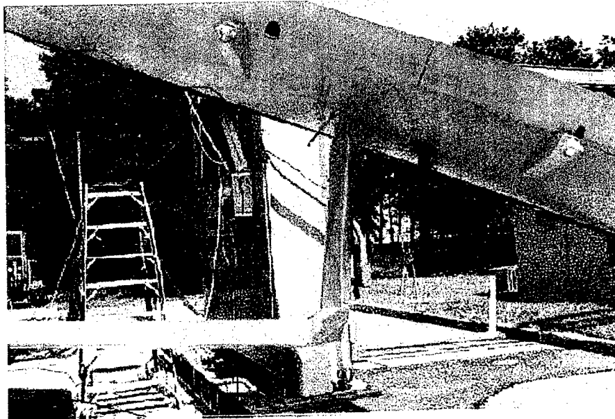
FIGURE 30. COPILOT-SIDE STRUT DEFORMATION POSTTEST
