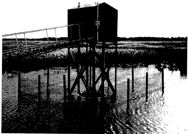
Figure 1. Telescoping weir operating at Craney Island CDF
