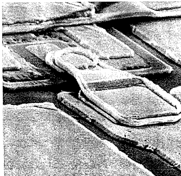
Fig. 3. Scanning Electron Microscopy picture of a RCE Schottky photodiode illustrating the air-bridge for top contact.
