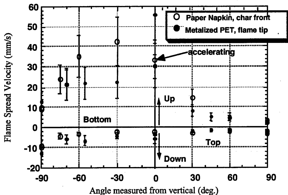
FIGURE 15. FLAME SPREAD VELOCITY
