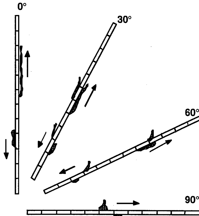
FIGURE 6b. OBSERVED FLAME LENGTHS ON PET FILM, INCREMENTS 2.5 cm
