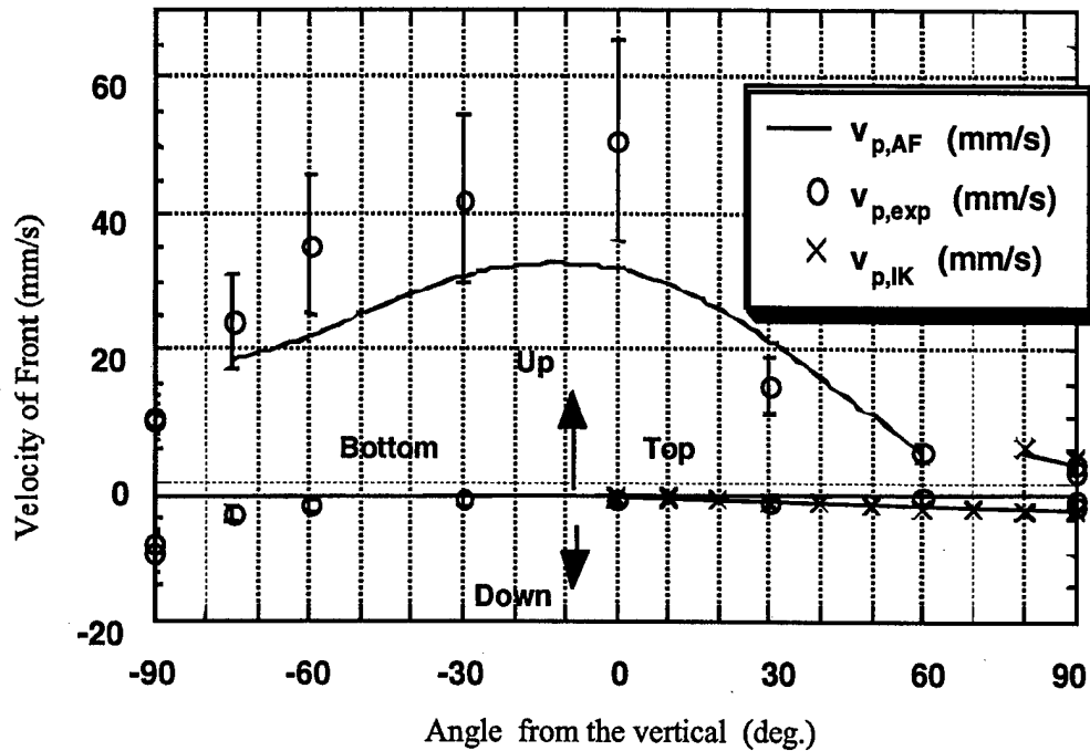
FIGURE 17. COMPARISON OF PREDICTED AND MEASURED FLAME SPEEDS FOR THE NAPKIN
