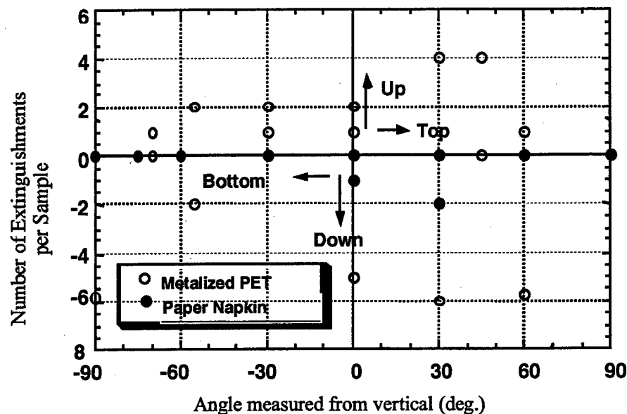
FIGURE 14. FREQUENCY OF EXTINGUISHMENT DURING FLAME SPREAD
