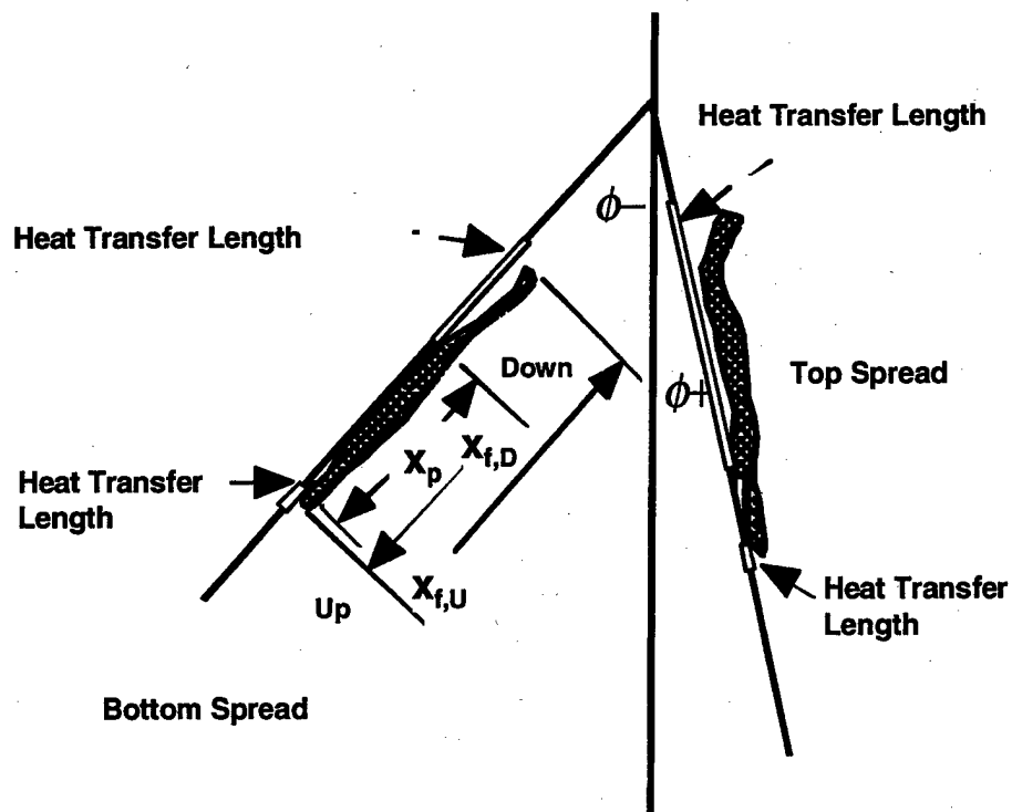
FIGURE 4. SPREAD CONFIGURATIONS AND THEORETICAL NOTATION
