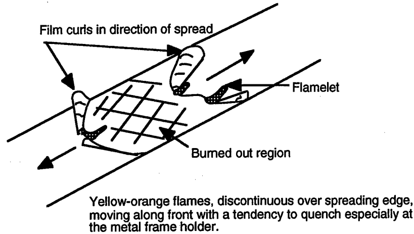
FIGURE 7b. FLAME SPREAD BEHAVIOR ON PET FILM
