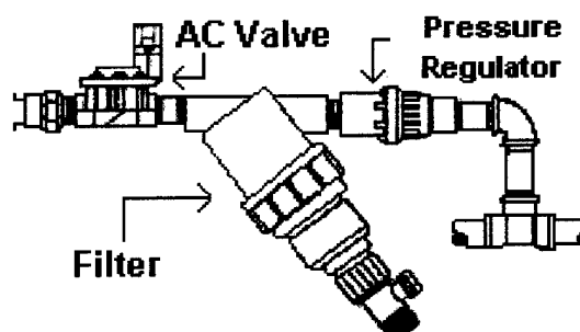
Figure 2. Filters are required for systems that utilize surface water sources and are recommended for all water sources
