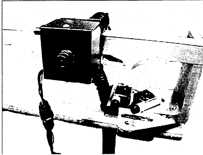
Figure 2. Close-up photograph of camera/carryage of gear driven rack. One set of positioning lasers appears to the lower right.
