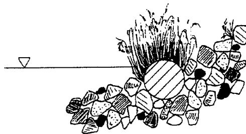
Figure 3. CGR shown at an appropriate elevation to sustain emergent plant growth (from Bestmann GmbH, Wedel, Germany)
