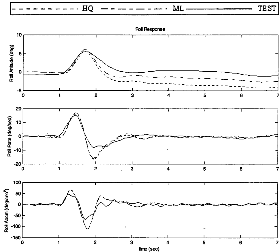
Figure 77 Flight 953-795 Run 092 On-Axis Response 22000, FSCG 360, 3000 ft DA
