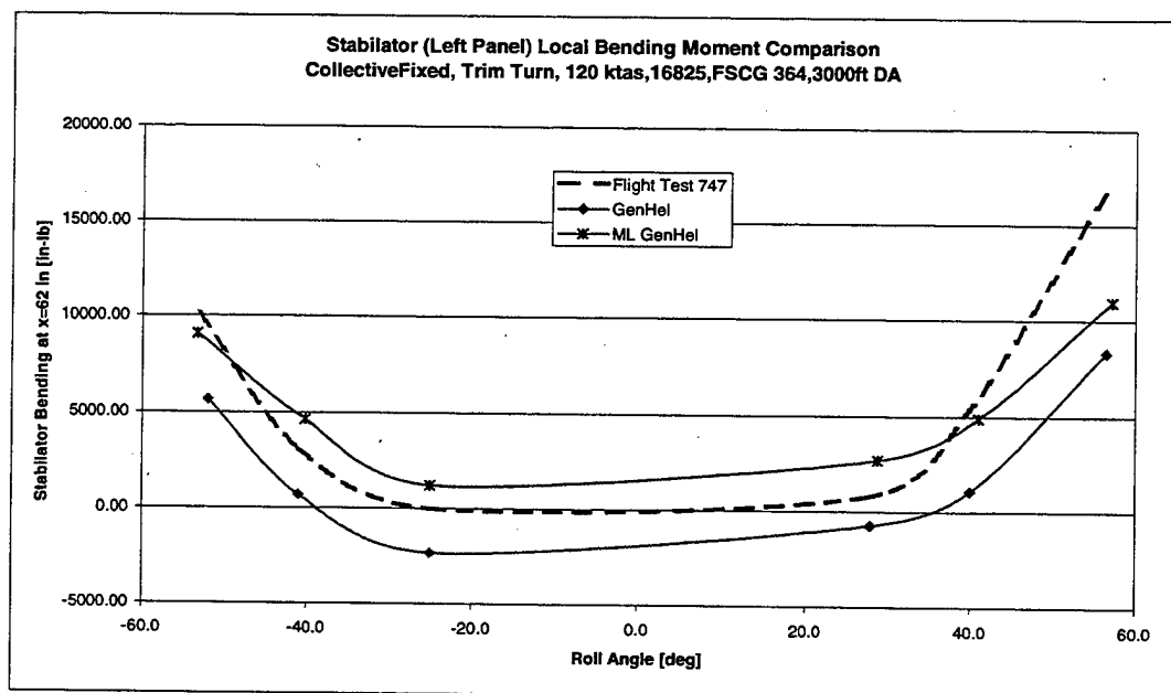
Figure 21 Trim Turn Stabilator Bending Comparison 16825 lb, FSCG 364 in, 3000 ft DA
