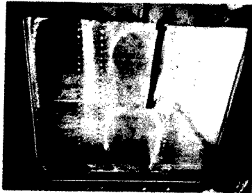
FIG. 23 NODE LINES OF FUNDAMENTAL MODES OF ALUMINUM AND VISCOELASTIC PANELS - SOFT SUSPENSION SYSTEM
