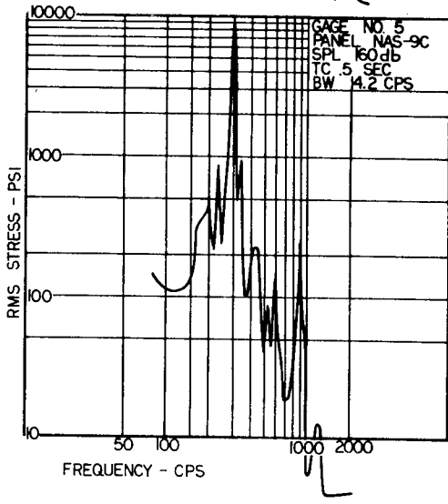
FIG.9 TYPICAL RMS STRESS RESPONSE AS A FUNCTION OF FREQUENCY AND PROBABILITY DENSITY ANALYSIS FOR ALL CONTROL PANEL AT THE 3 TEST SPL
