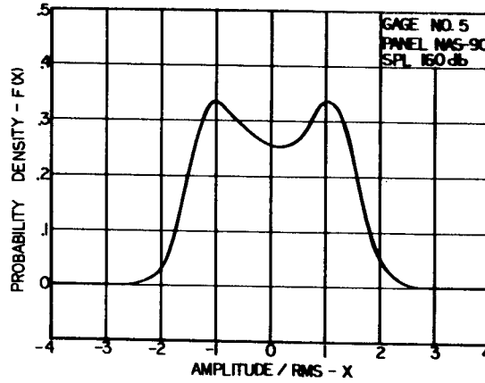
FIG.9 TYPICAL RMS STRESS RESPONSE AS A FUNCTION OF FREQUENCY AND PROBABILITY DENSITY ANALYSIS FOR ALL CONTROL PANEL AT THE 3 TEST SPL
