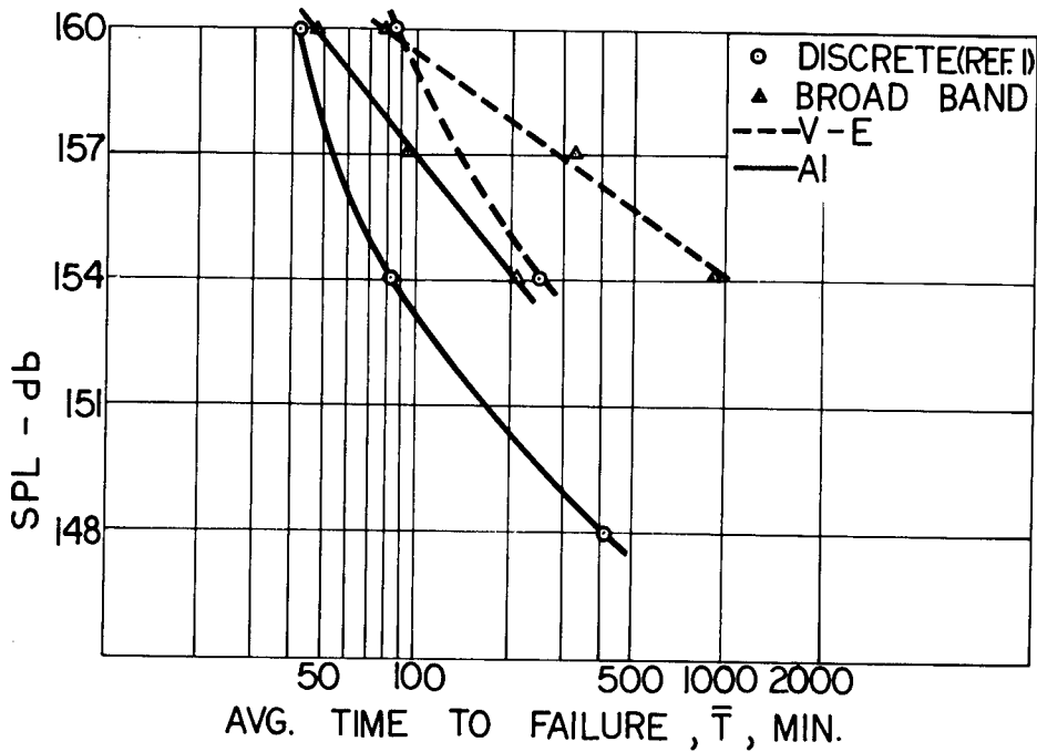
FIG. 15 COMPARISON OF PANEL FATIGUE LIFE AT DISCRETE AND BROAD BAND TESTING
