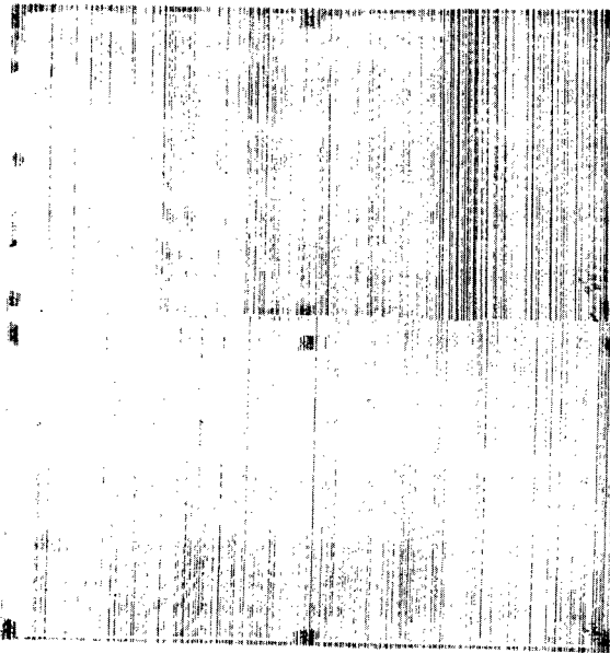
BOND VOID NEAR EDGE
