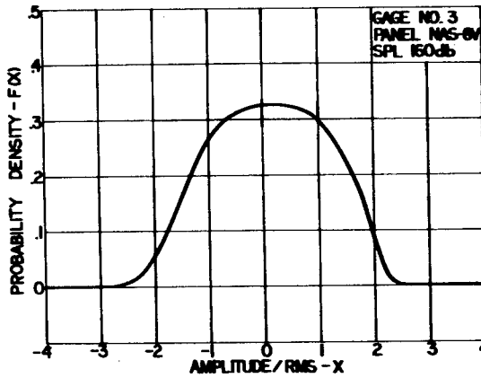
FIG. 10 TYPICAL RMS STRESS RESPONSE AS A FUNCTION OF FREQUENCY AND PROBABILITY DENSITY ANALYSIS FOR AL CONTROL PANEL AT THE 3 SPL
