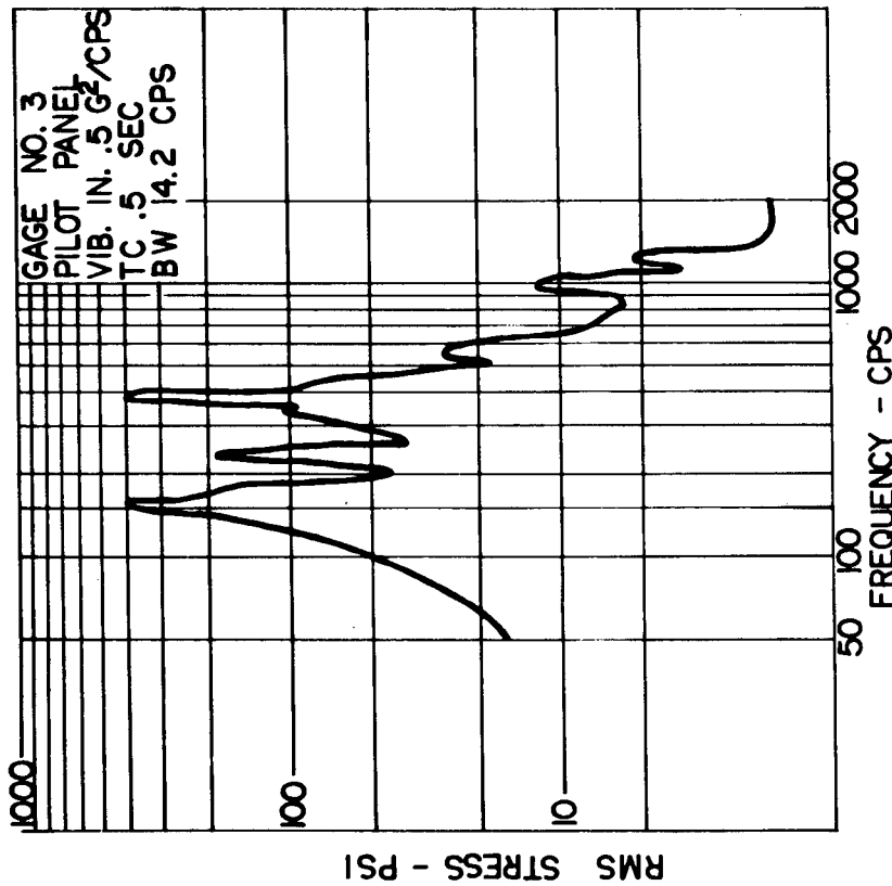
FIG. 18 RMS STRESS RESPONSE OF VISCOELASTIC PANEL DURING SHAKER EXCITATION
