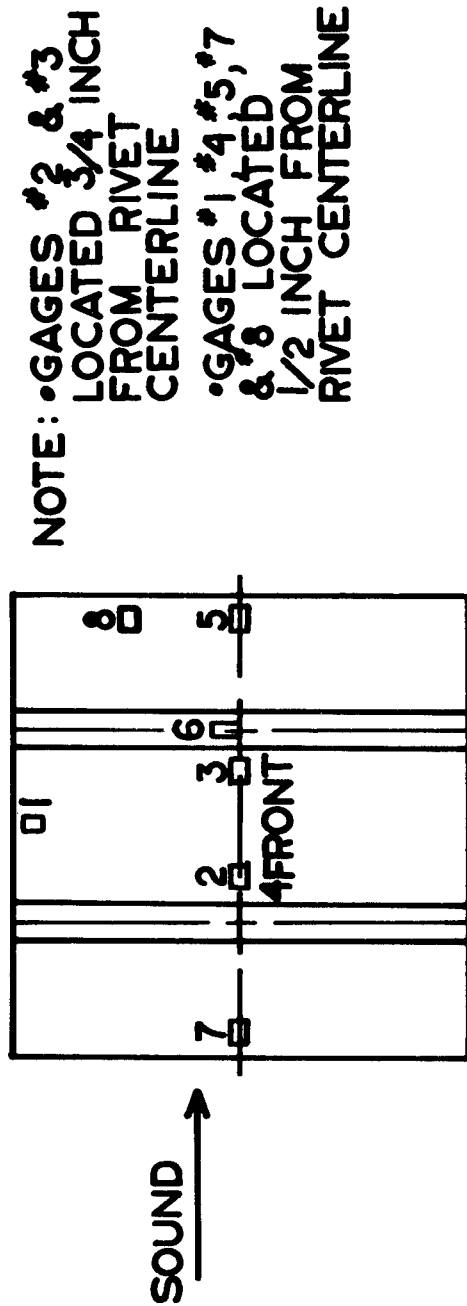
FIG. 5 STRAIN GAGE LOCATION AND DESIGNATION BACK SIDE OF PANEL
