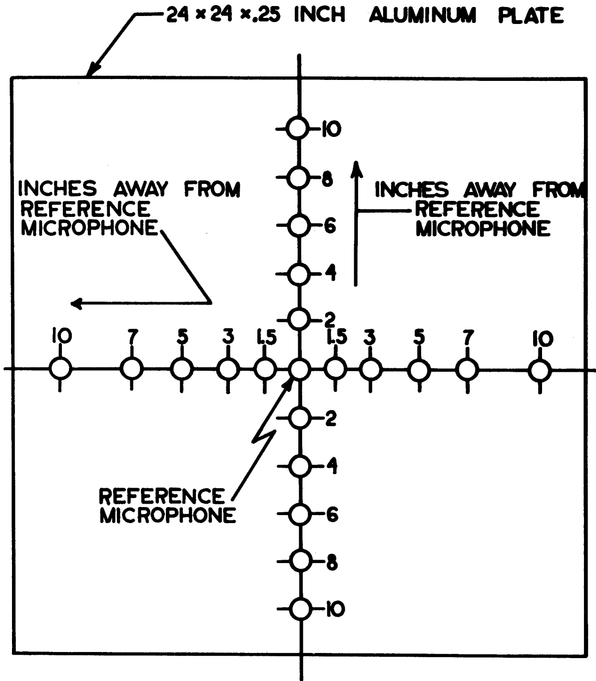
FIG.20 MICROPHONE POSITIONS IN DUMMY PANEL FOR CORRELATION MEASUREMENTS
