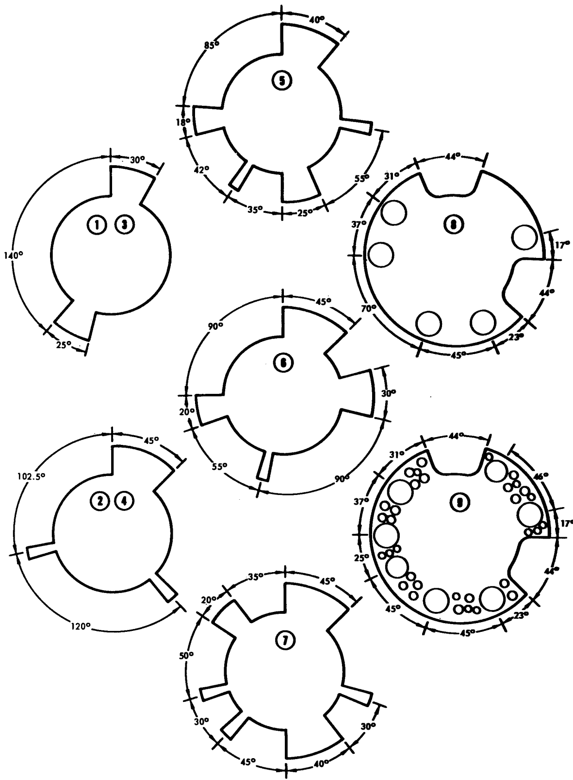
FIG. 3 ROTOR SHAPES
