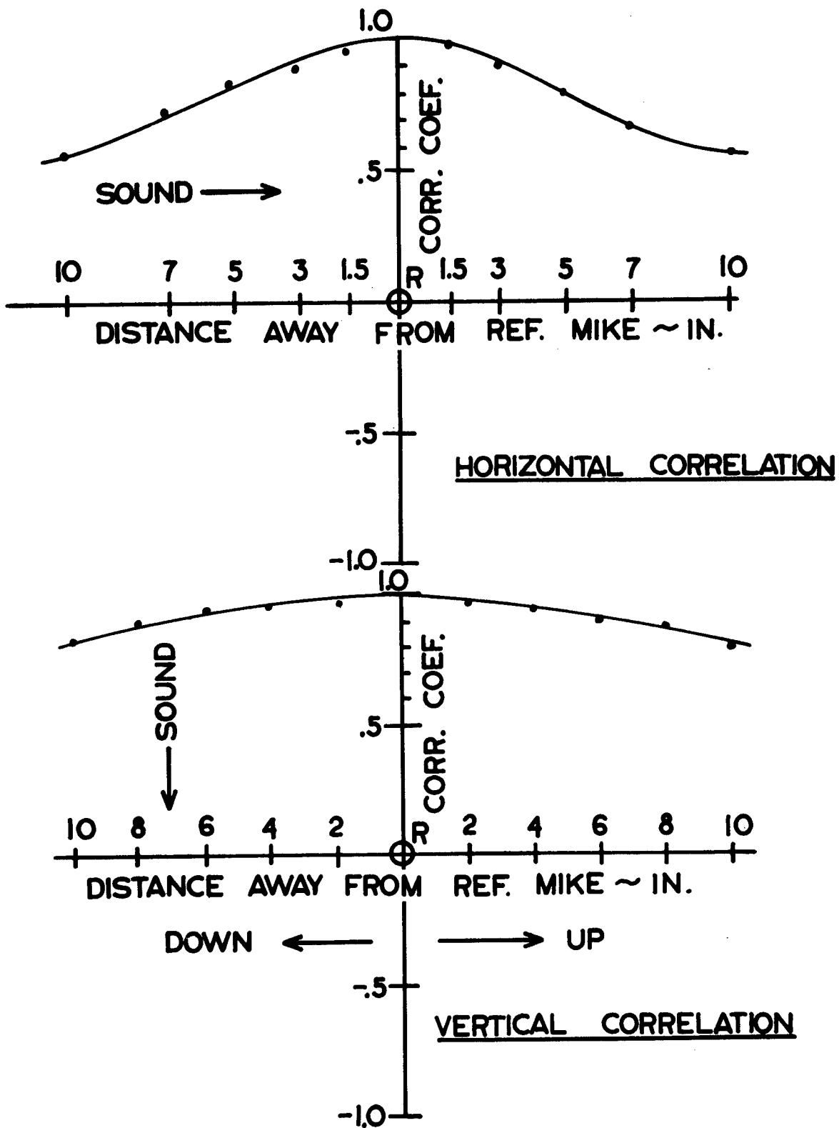
FIG. 22 CORRELATION MEASUREMENTS ACROSS A DUMMY PANEL
