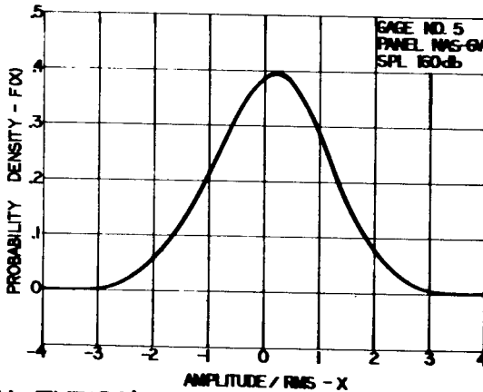
FIG. II TYPICAL RMS STRESS RESPONSE AS A FUNCTION OF FREQUENCY AND PROBABILITY DENSITY ANALYSIS FOR V-E PANEL AT THE 3 SPL
