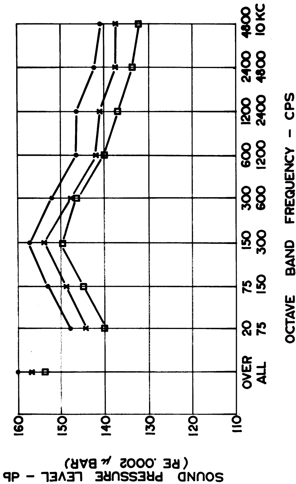
FIG. 14 OCTAVE BAND ANALYSIS OF TEST LEVELS
