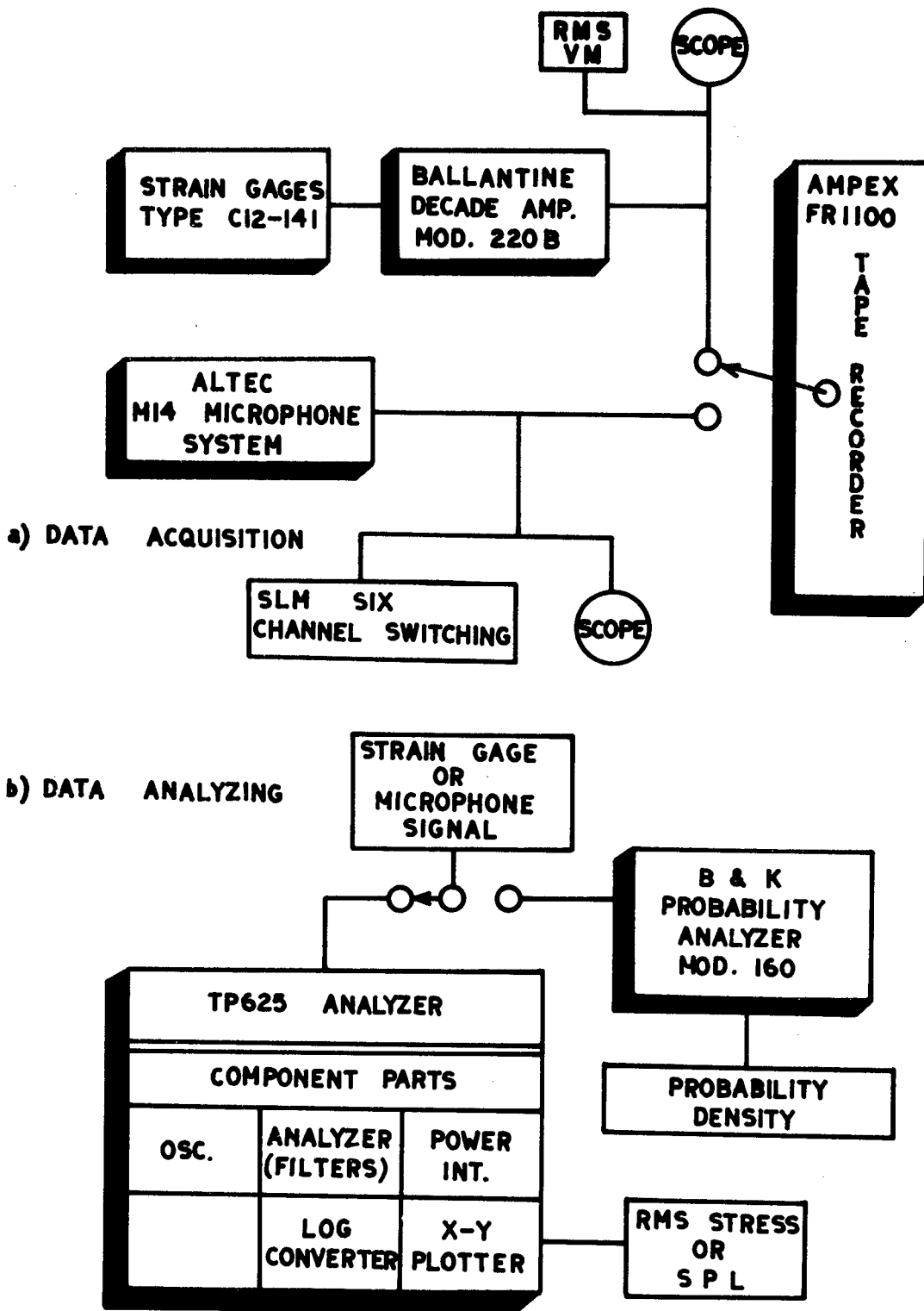
FIG. 6 BLOCK DIAGRAM OF DATA PROCESSING SYSTEM
