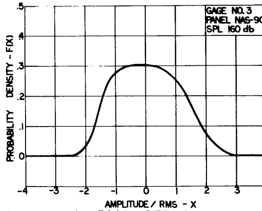
FIG. 12 TYPICAL RMS STRESS RESPONSE AS A FUNCTION OF FREQUENCY AND PROBABILITY DENSITY ANALYSIS FOR V-E PANEL AT THE 3 SPL
