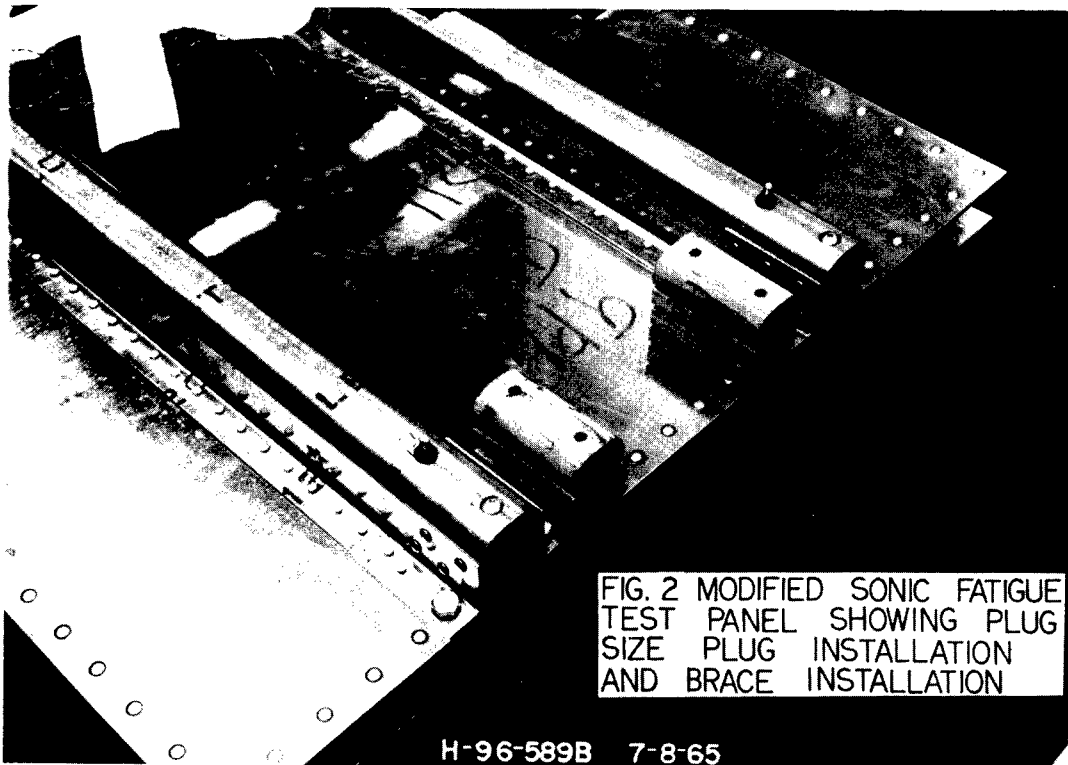
FIG. 1 PANEL INSTALLATION IN STRUCTURAL FRAME
