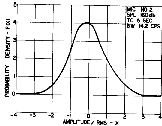
FIG. 13 NARROW BAND AND PROBABILITY DENSITY ANALYSIS OF THE NOISE SOURCE (BROAD BAND SIREN)
