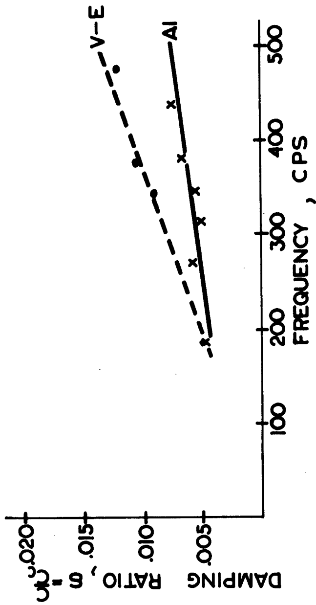
FIG. 24 DAMPING RATIO OF VISCOELASTIC AND AI PANELS - HARD MOUNT
