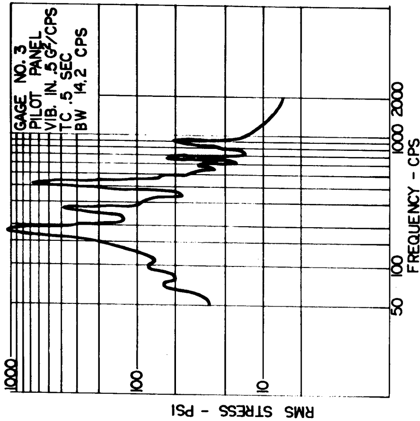
FIG. 19 RMS STRESS RESPONSE OF ALUMINUM CONTROL PANEL DURING SHAKER EXCITATION
