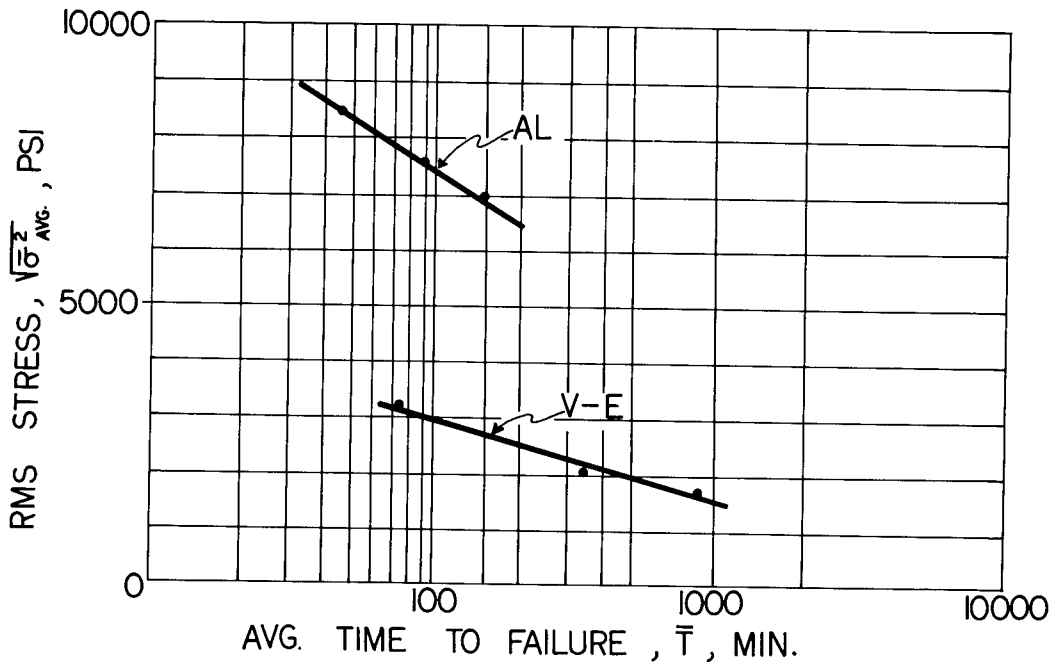
FIG. 16 FATIGUE LIFE OF VISCOELASTIC AND ALUMINUM PANELS AS A FUNCTION OF THE AVERAGE ROOT-MEAN-SQUARE STRESS AT THE PREDOMINATE RESPONSE FREQUENCY FOR RANDOM LOADING (14.2 CPS BW)
