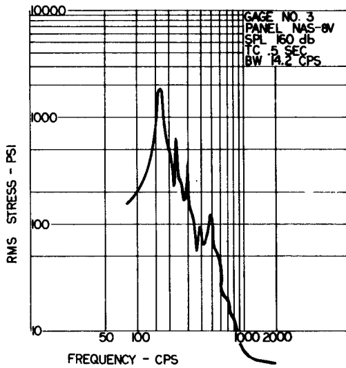
FIG. 10 TYPICAL RMS STRESS RESPONSE AS A FUNCTION OF FREQUENCY AND PROBABILITY DENSITY ANALYSIS FOR AL CONTROL PANEL AT THE 3 SPL
