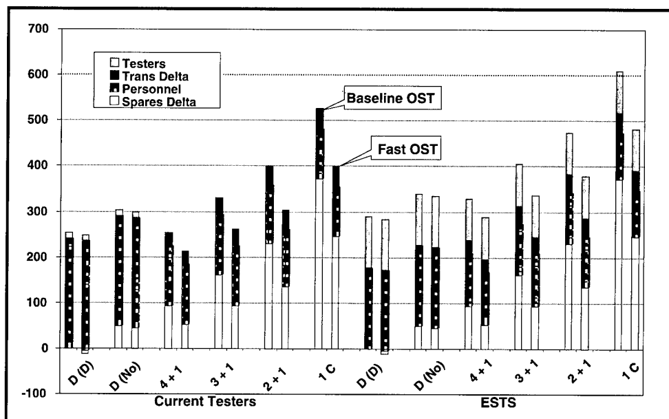
Figure 2. Total Cost by Structure, OST, and Tester Configuration
