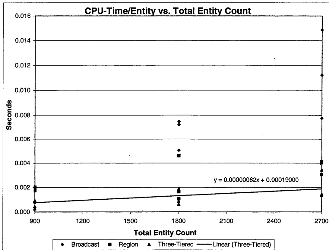
Figure 20. CPU-Time Per Entity of Interest vs. Total Entity Count
