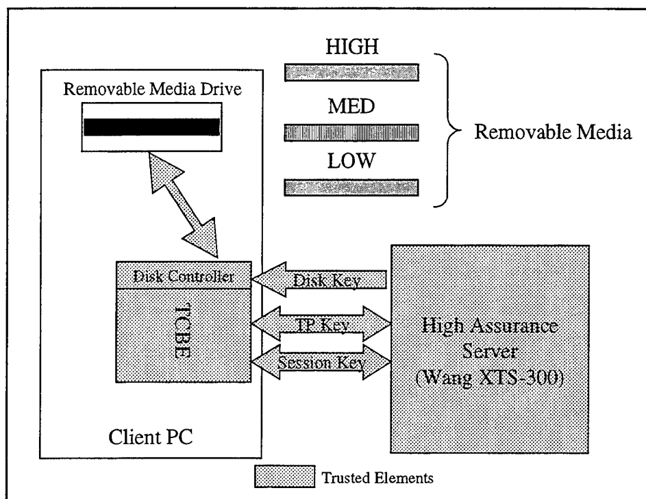
Figure 5. Operating System Delivery via Removable Media
