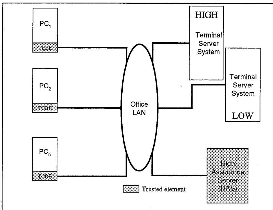
Figure 16. Multiple TSEs for Separate Classifications
