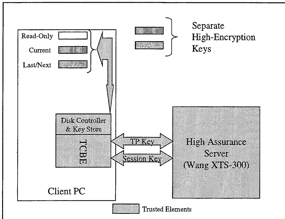
Figure 10. Multiple Disks with Ghosting Technology
