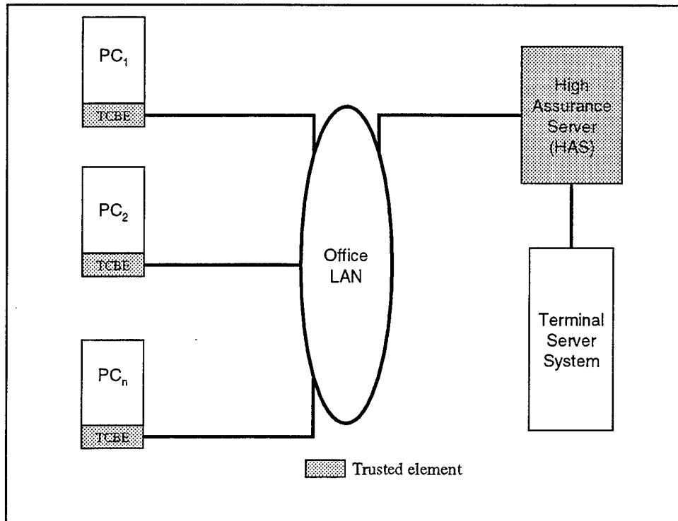
Figure 14. TSE and HAS in Series
