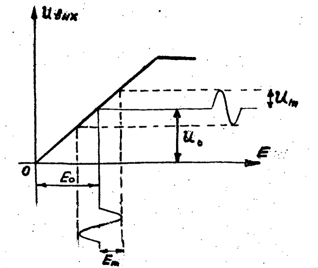
Figure 7. Obtaining Modulated Voltage at the Output of the Photo-detector With Sine-Wave Modulation
