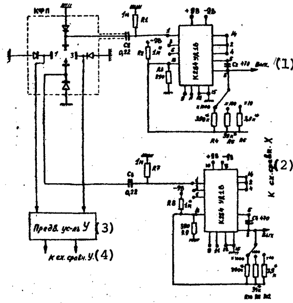
Figure 4. Schematic Diagram of Coordinate Photodetector (KFP) and Preamplifier
