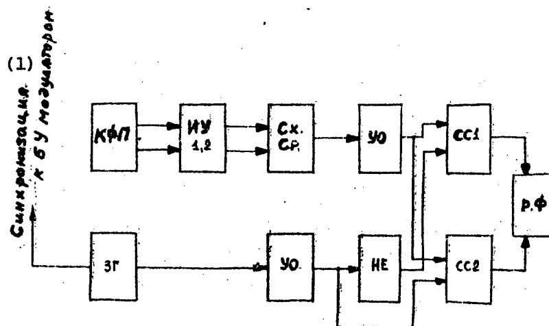
Figure 8. Block Diagram of Instruction Block With Sine-Wave Modulation of Optical Radiation
