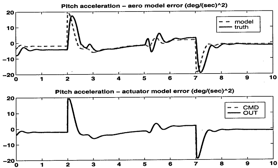
Figure 4.61: Mach 0.35, 5000 ft. Altitude, Min Signature CA Mode
