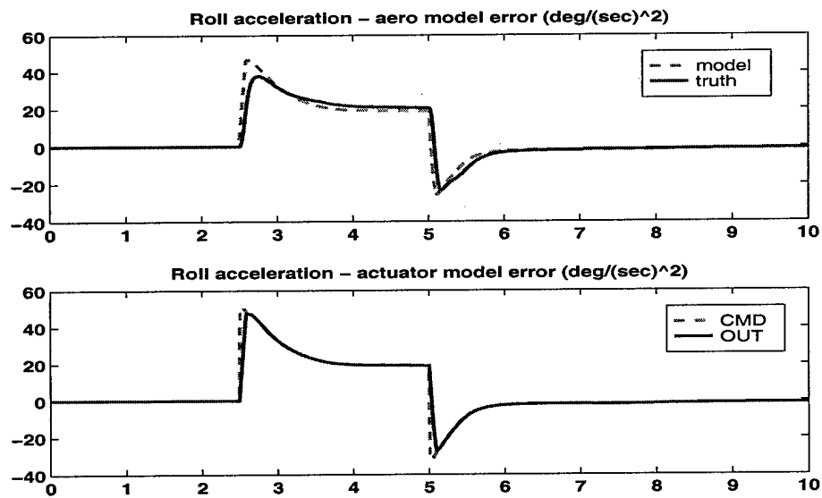
Figure 4.27: Mach 0.35, 5000 ft. Altitude, Min Def CA Mode
