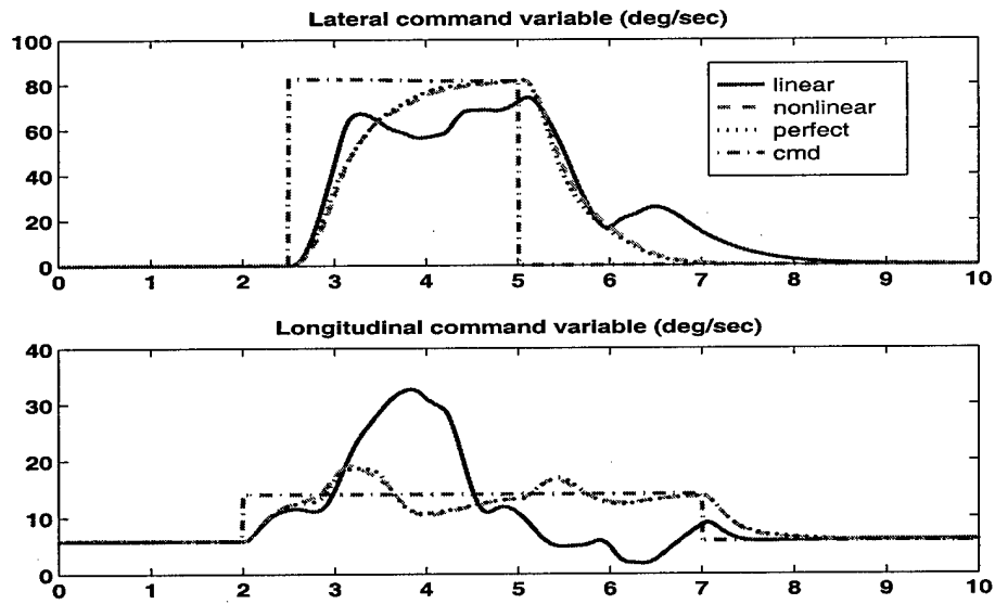
Figure 3.5: Mach 0.35, 5000 ft. Altitude, Min Vec CA Mode
