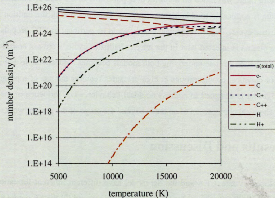
Figure 1. SE Model Calculations of Reaction Product Number Densities vs. Temperature for a 50-bar Gas Formed From Decomposed Polyethylene.
