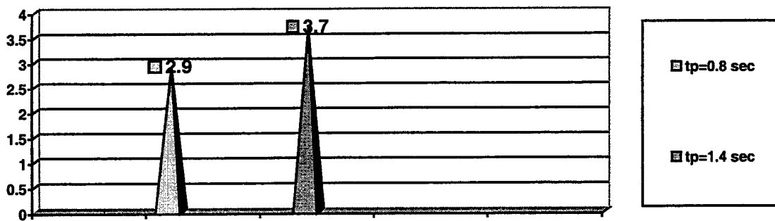
Figure 6.4 S/N for various t_p
