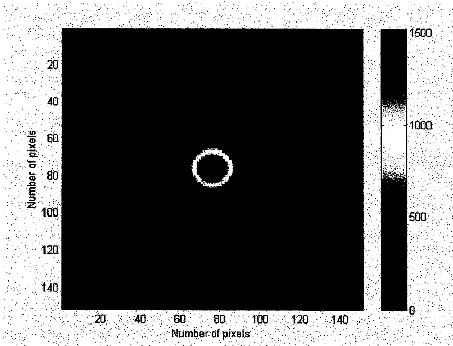
Figure 7.3 The pyrophoric image at t=t_p=1.5 sec.
