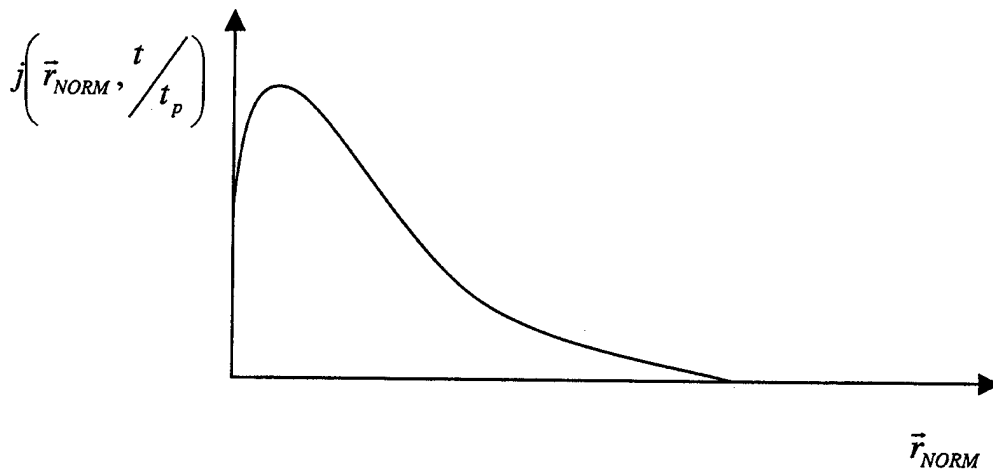
Figure 3.8 Pyrophoric Space distribution for one instant of time t .
