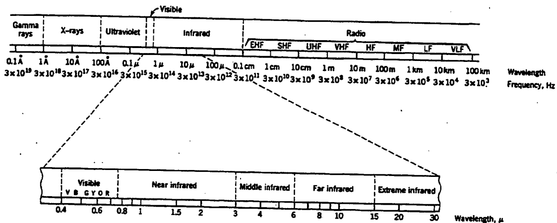
Figure 2.1 The Electromagnetic Spectrum. (From Ref [1])
