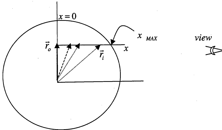
Figure 3.9 The integrated pyrophoric model projection
