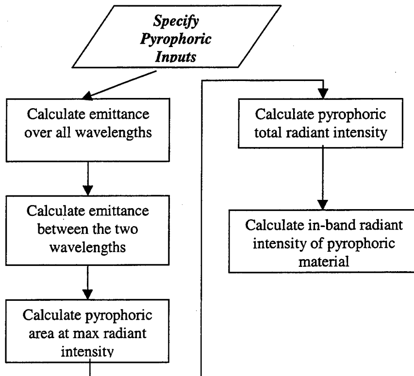
Figure 3.2 Calculation of In-Band Radiant Intensity.
