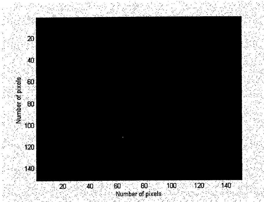
Figure 7.1 The Plume Image.
