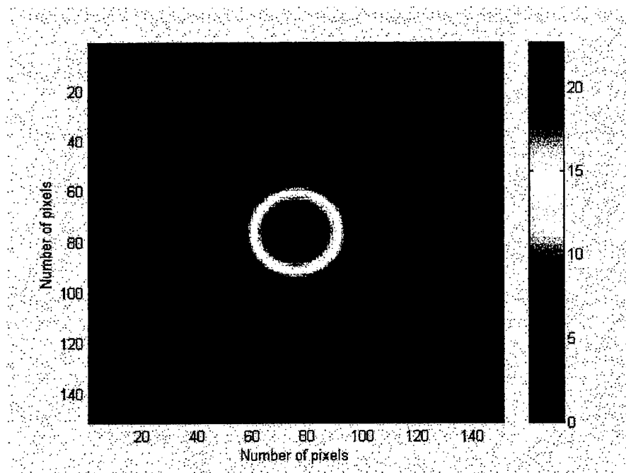
Figure 7.6 The pyrophoric image at t=7 sec.
