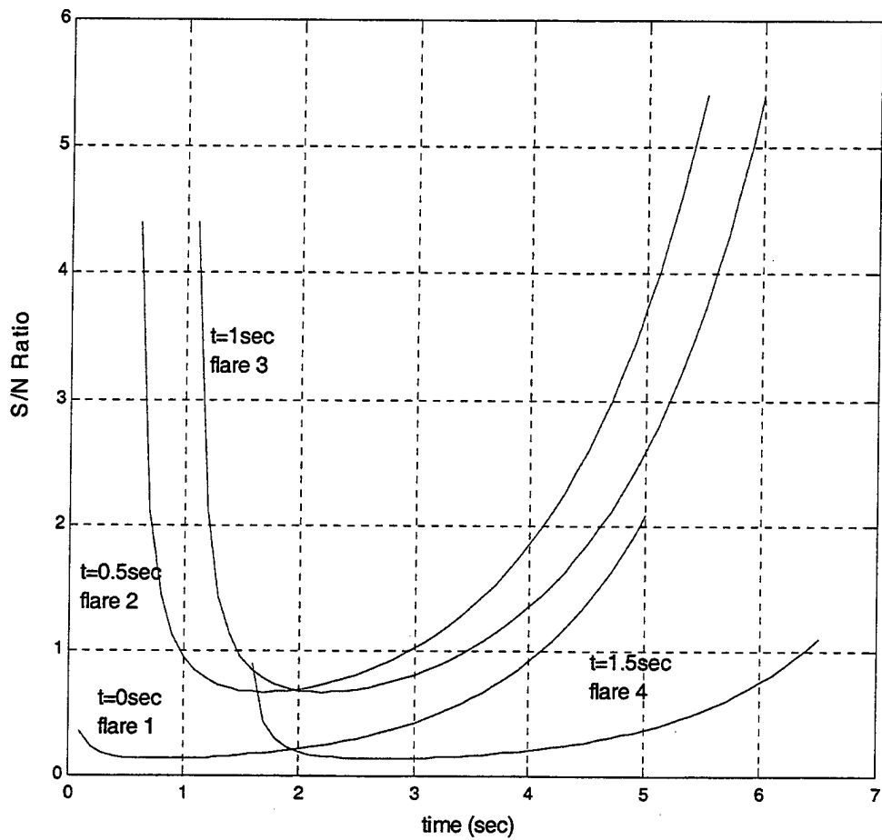
Figure 8.5 S/N ratio Curves for Each Flare.
