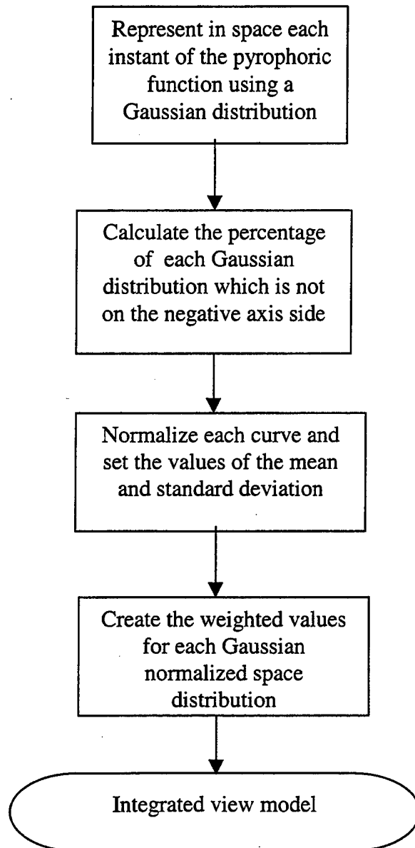
Figure 3.5 Normalized Space Distribution Structure
