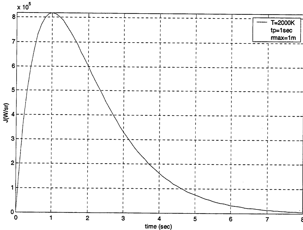
Figure 3.4 The Time Radiant Intensity Distribution of Pyrophoric Burn
