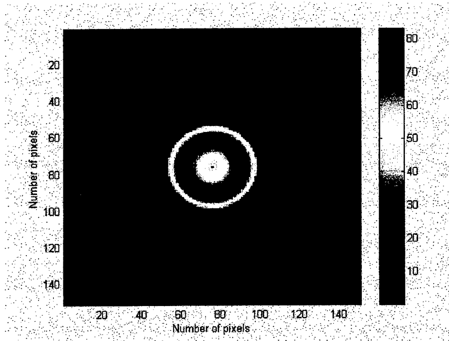
Figure 7.5 The pyrophoric image at t=5 sec.
