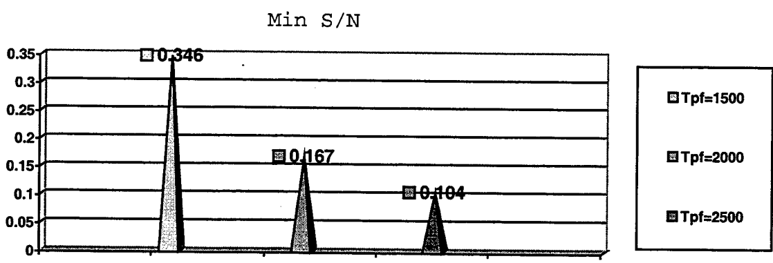
Figure 6.1 S/N for various T_{pf}
