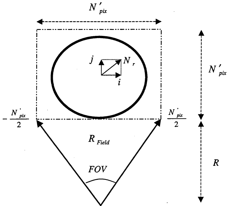
Figure 5.5 Pyrophoric Image Construction.
