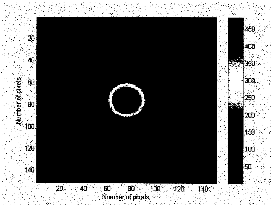
Figure 7.4 The pyrophoric image at t=3 sec.
