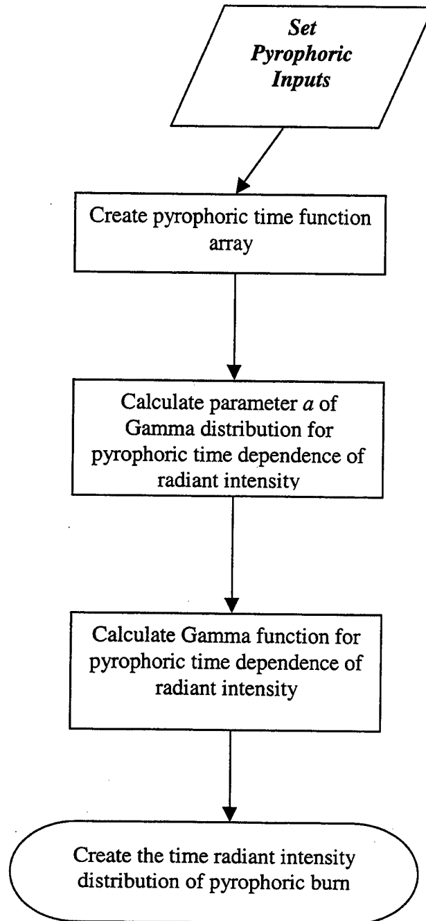
Figure 3.3 The Time Radiant Intensity Distribution Structure of Pyrophoric Burn.
