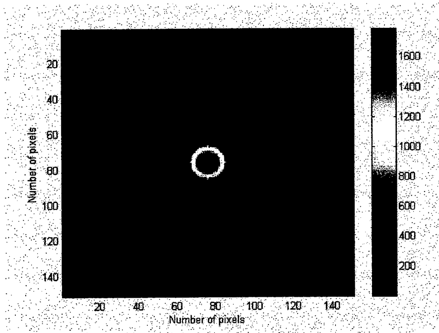
Figure 7.2 The pyrophoric image at t=1 sec.
