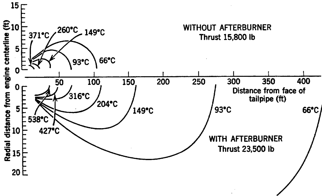
Figure 4.1 Exhaust Temperature Contours for a JT4A Turbojet Engine with and without Afterburner (From Ref [1])
