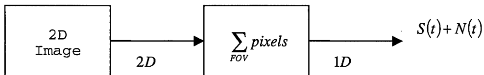
Figure 7.7 Reticle based Detection System.
