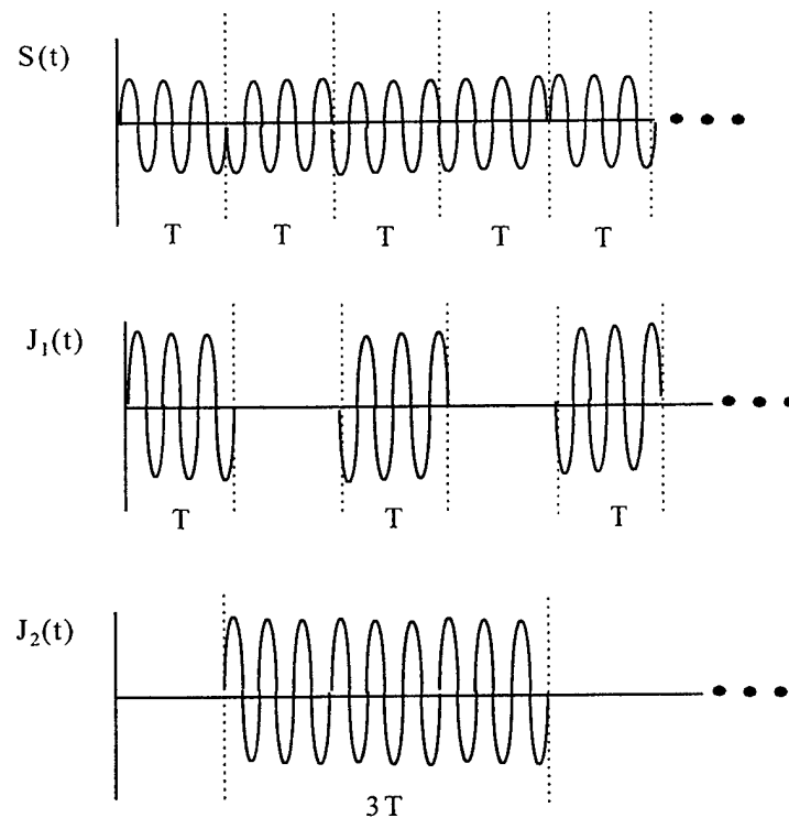
Figure 2.6 Pulsed Jamming
