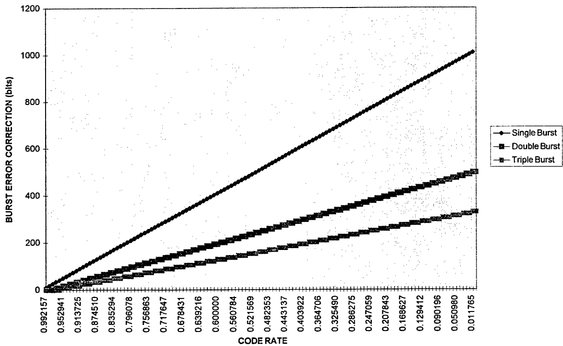
BURST ERROR CORRECTING CAPABILITY (Reed-Solomon Codes of Length n = 255 )
