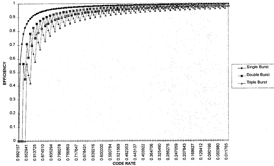
BURST ERROR CORRECTION EFFICIENCY (Reed-Solomon Codes of Length n = 255 )
