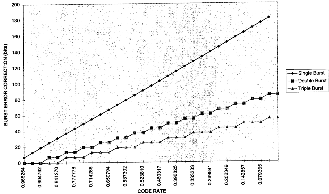
BURST ERROR CORRECTING CAPABILITY (Reed-Solomon Codes of Length n = 63 )
