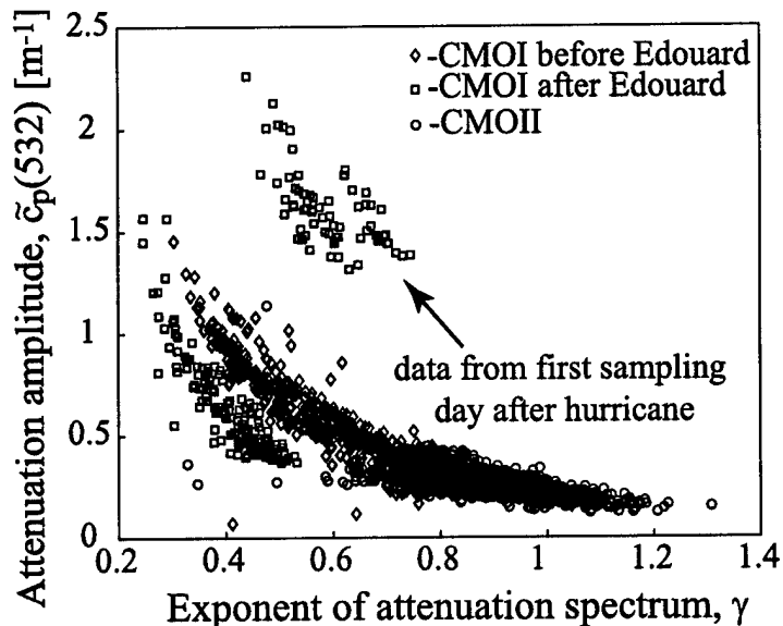
Figure 3. Particulate attenuation vs. its hyperbolic slope measured within the BBL during the two CMO sampling seasons. Both were derived by least-square fitting the particulate attenuation to:
