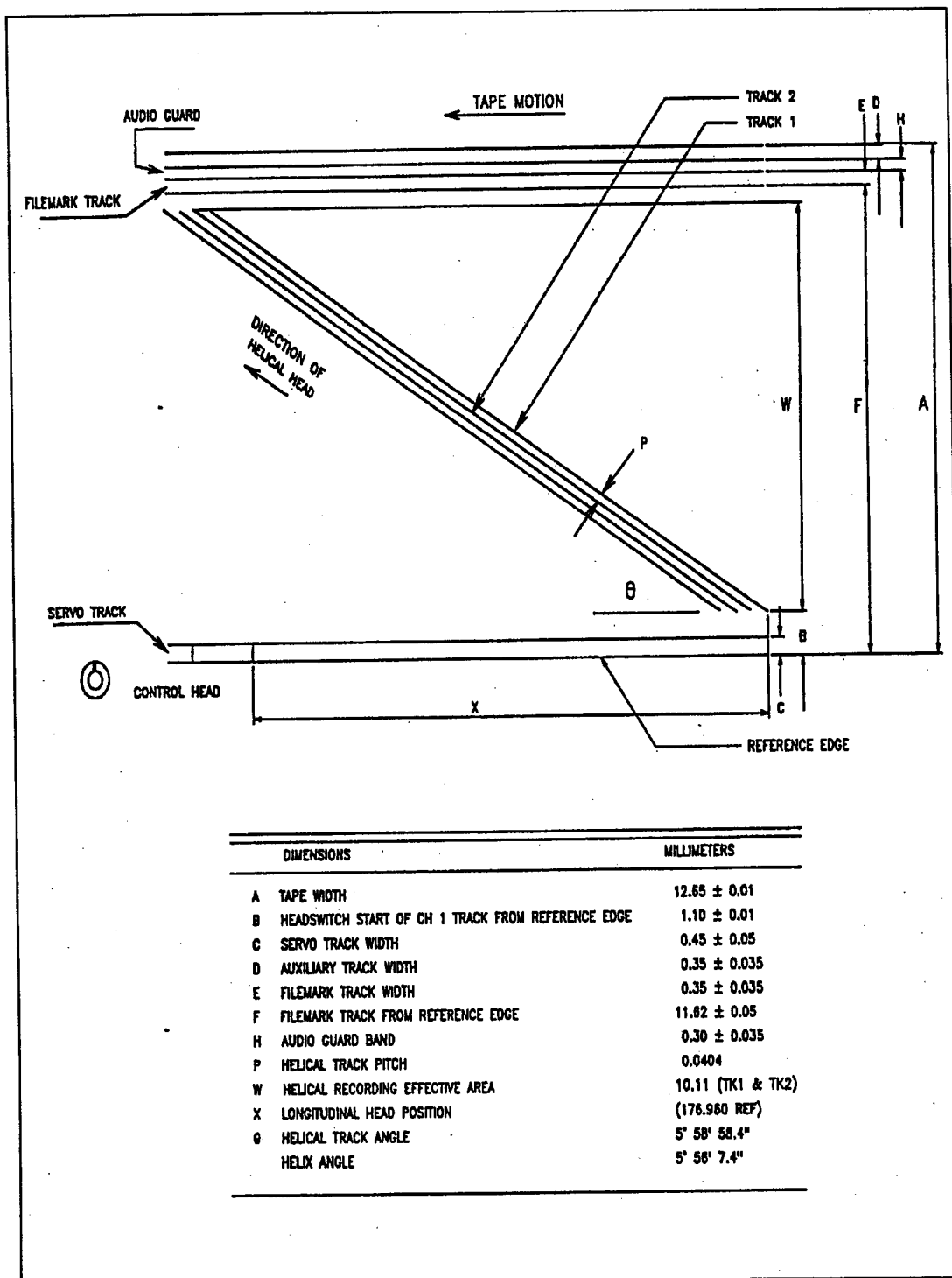
Figure 6-12. Recorded tracks on tape, B format.
