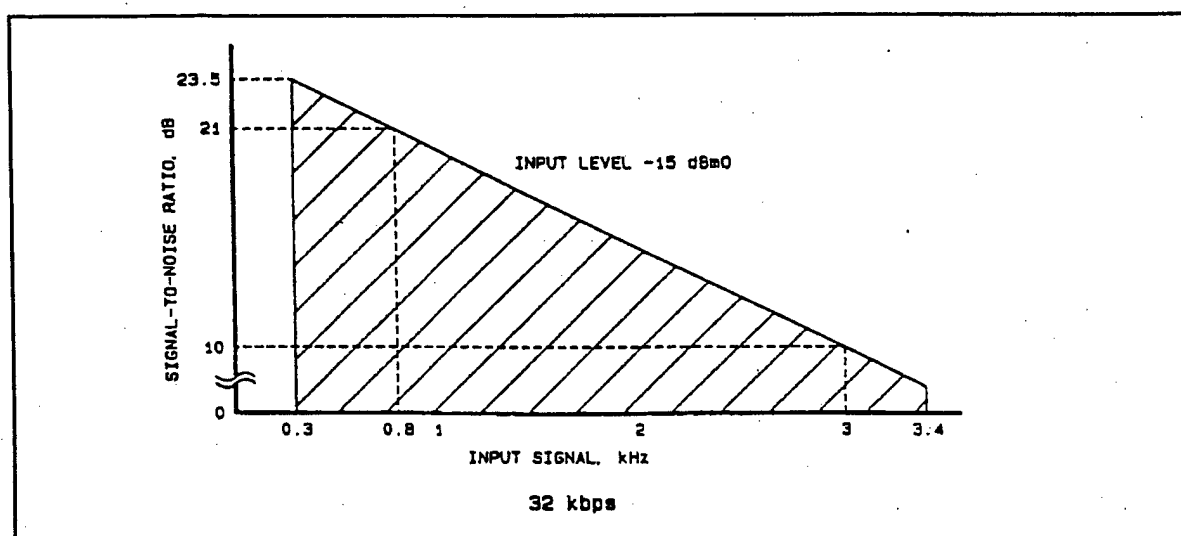
Figure F-7b. Signal to quantizing noise ratio versus frequency for CVSD (32 kbps).
