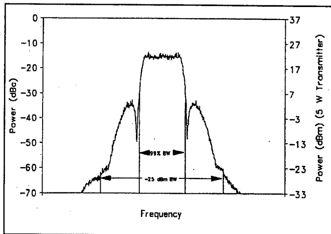
Figure A-2. RNRZ PCM/FM signal.
