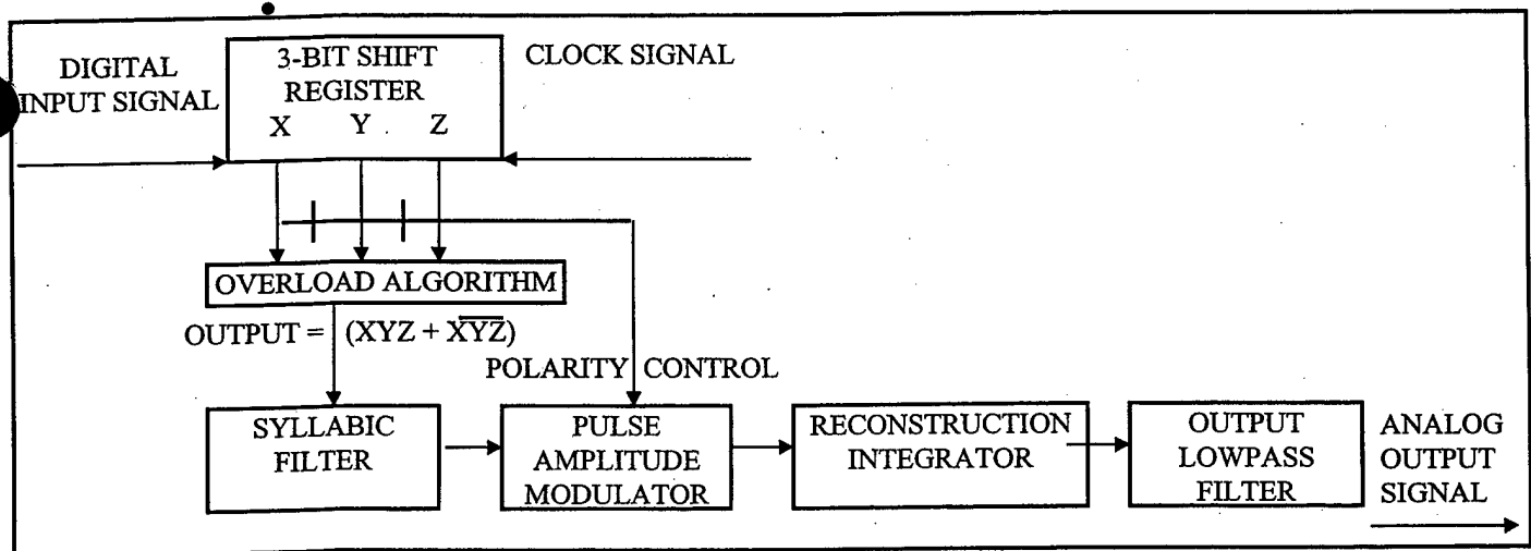
Figure F-1b. Typical CVSD decoder.
