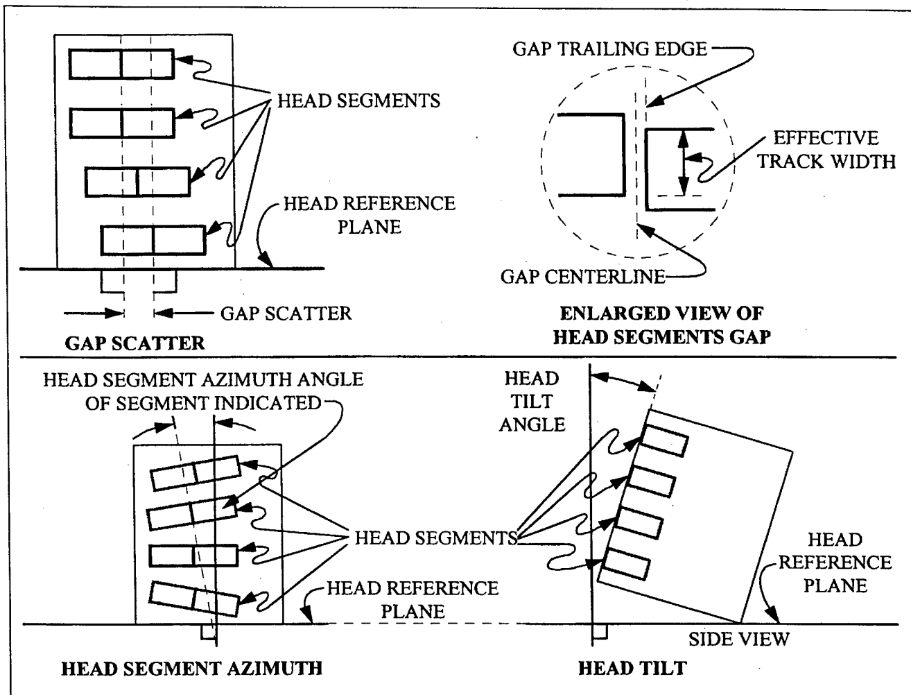
Figure 6-3. Head and head segment mechanical parameters.
