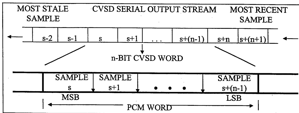
Figure 5-1. Insertion of CVSD encoded audio into a PCM stream.
