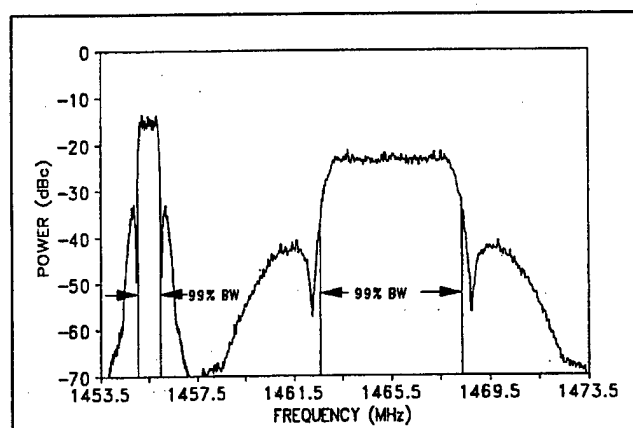
Figure A-1. 800-kb/s and 5-Mb/s RNRZ PCM/FM signals.
