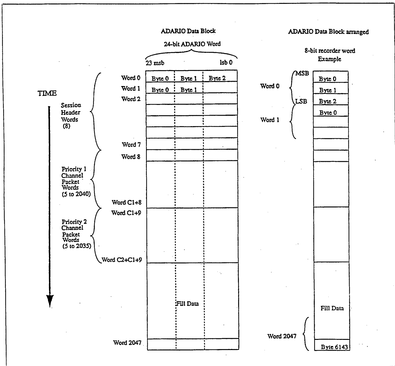
Figure G-2. ADARIO data blocks.
