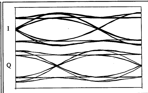
Figure A-13. FQPSK-B I & Q eye diagrams (at input to IQ modulator).
