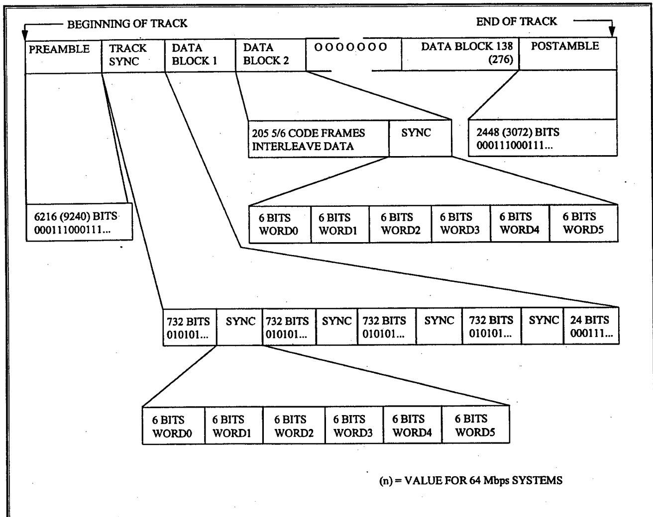
Figure 6-14. Helical Track Format.
