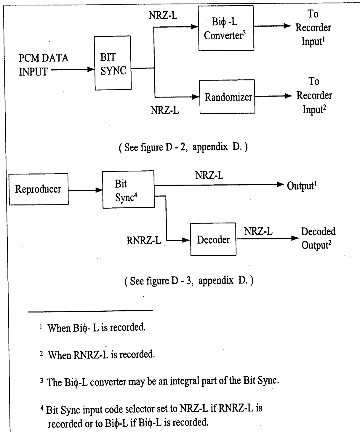
Figure 6-5. Serial high-density digital record and reproduce.
