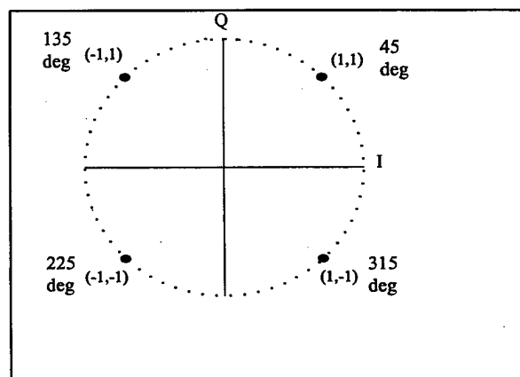
Figure A-11. I & Q constellation.
