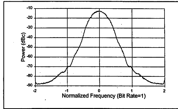
Figure A-15. FQPSK-B spectrum with random input data.
