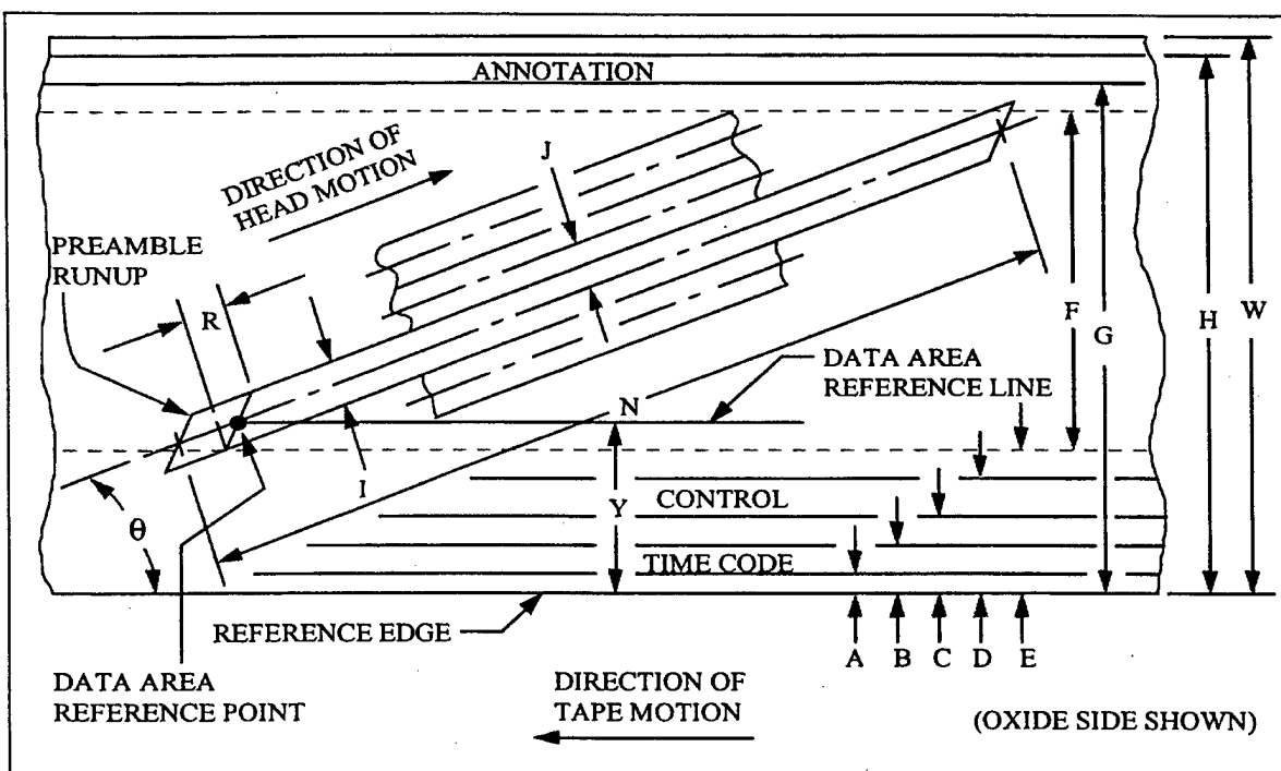
Figure 6-6. Location and dimensions of recorded tracks.
