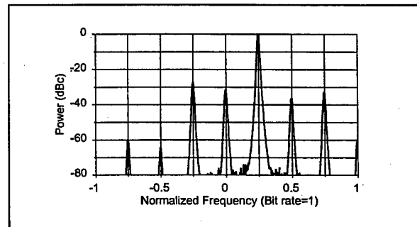
Figure A-16. FQPSK-B spectrum with all 1's input and large modulator errors.
