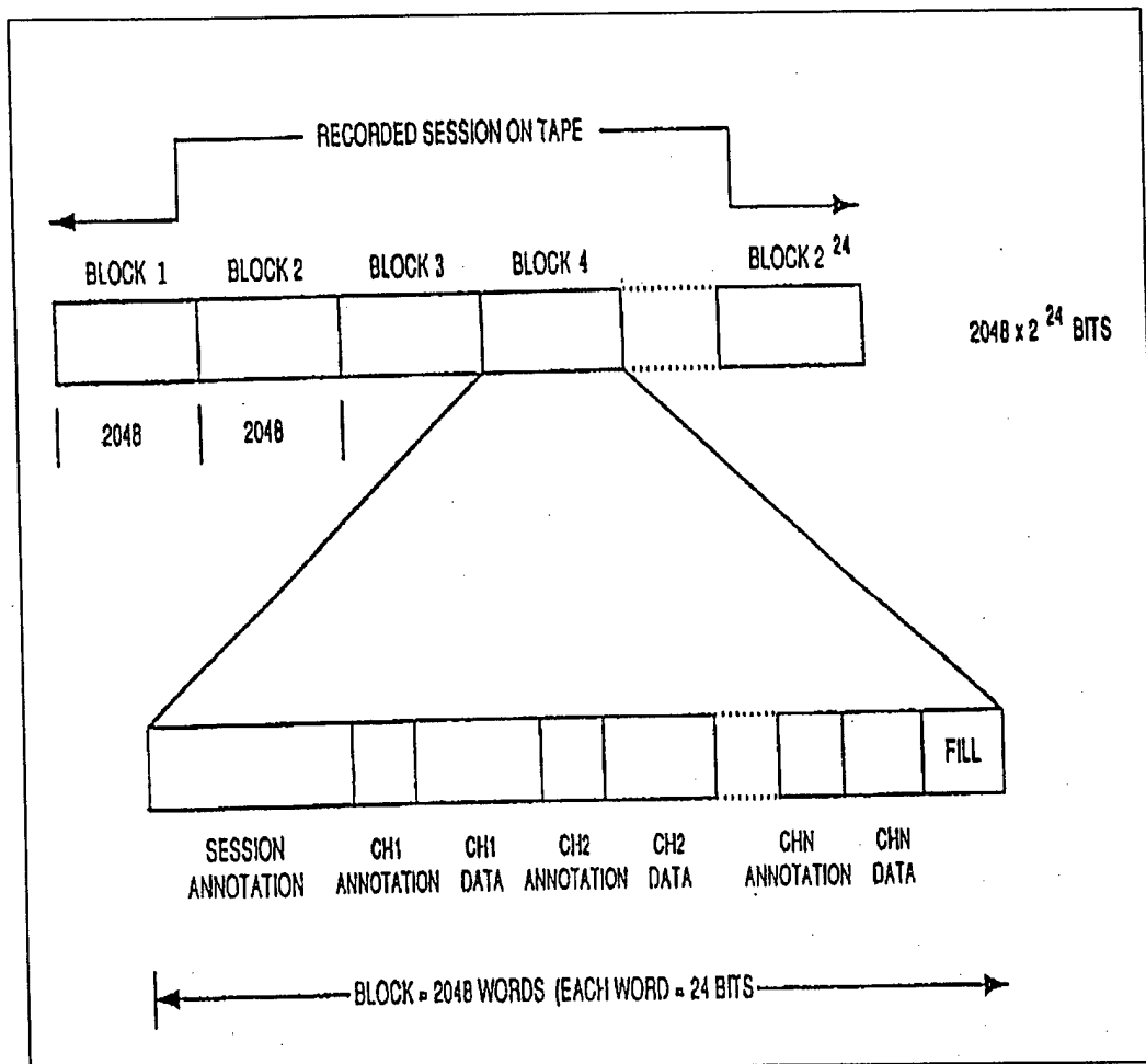
Figure 6-7. ADARIO block format.
