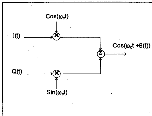
Figure A-10. OQPSK modulator.
