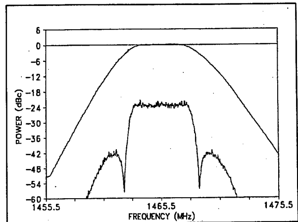
Figure A-3. Spectrum analyzer calibration of 0-dBc level.
