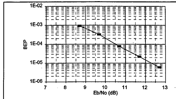
Figure A-17. FQPSK-B BEP vs E_b/N_0 .
