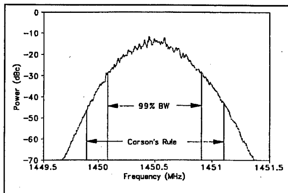
Figure A-5. FM/FM signal and Carson's Rule.
