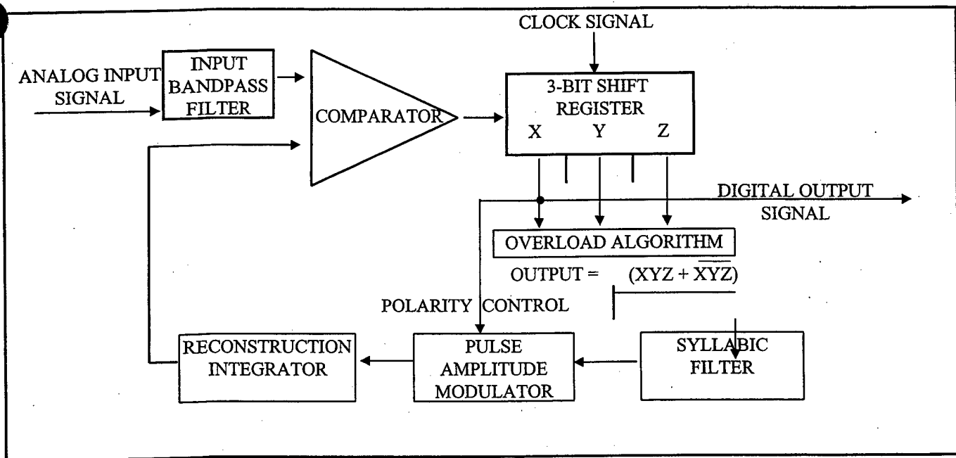
Figure F-1a. Typical CVSD encoder.
