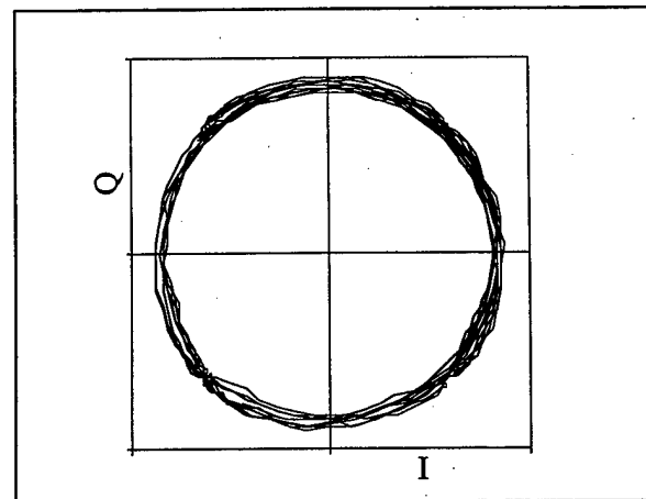
Figure A-14. FQPSK-B vector diagram.
