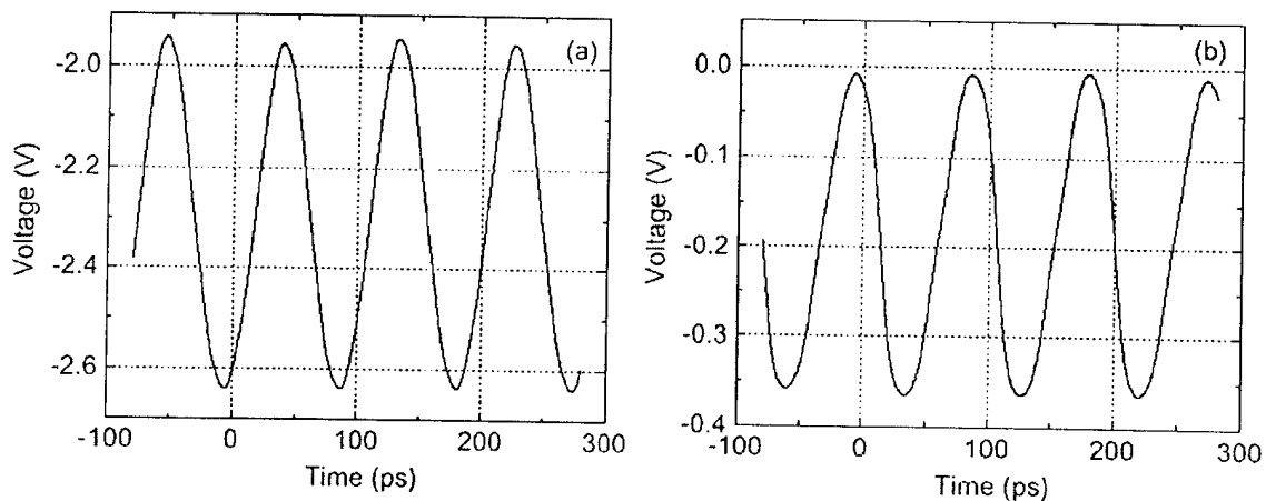
Figure 24. Sinusoidal microwave input of 10.56 GHz, (a) measured at position (A), (b) measured waveform at position (B)
