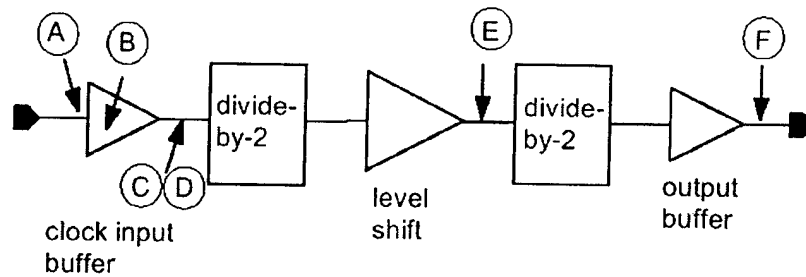
Figure 23. Block diagram of example digital circuit.
