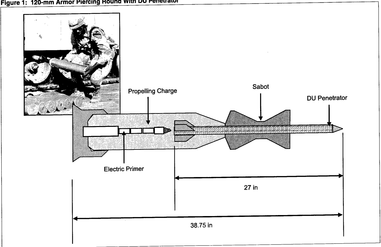
Figure 1: 120-mm Armor Piercing Round With DU Penetrator
