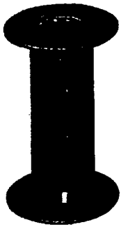
S-146 Spool —70 mm x 15 ft, flange diameter 1.719 in., core diameter 31/32 in. Round center hole with double keyways in both flanges.
