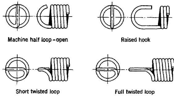
FIGURE 8-6 Types of ends used on extension springs. (Courtesy of Associated Spring Corporation.)
