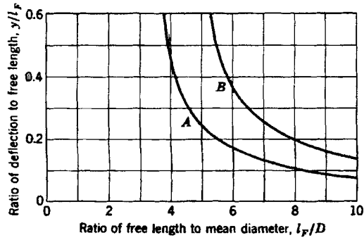
FIGURE 8-5 Curves show when buckling of compression coil springs may occur. Both curves are for springs having squared and ground ends. For curve A one end of the spring is compressed against a flat surface, the other against a rounded surface. For curve B both ends of the spring are compressed against flat and parallel surfaces.
