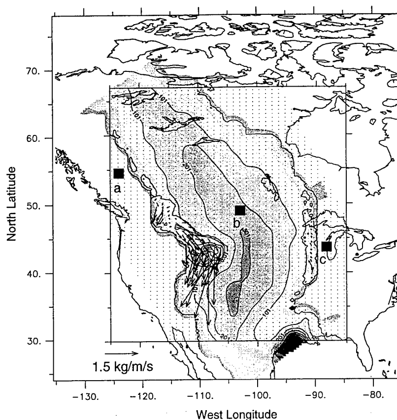
Fig. 6.—Net direction and magnitude of transport of suspended load (kg/m/s) during the eight days of the storm. Values reflect integration of sediment concentration over the lower 10 m of the water column times wind-driven current speed in lowest layer of POM expressed as kg per unit width per unit time.
