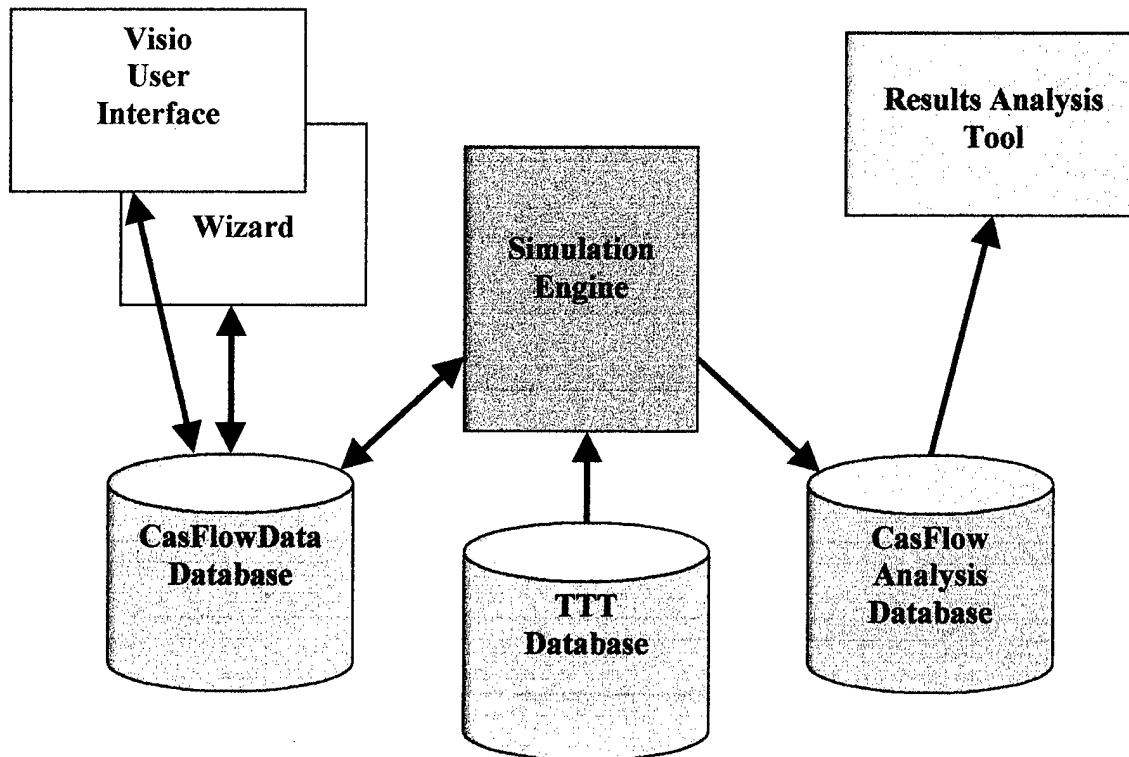
Figure 4-3 CasFlow Architecture
