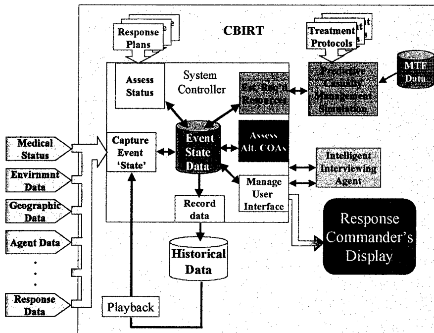
Figure 6-2 CBIRT Architecture
