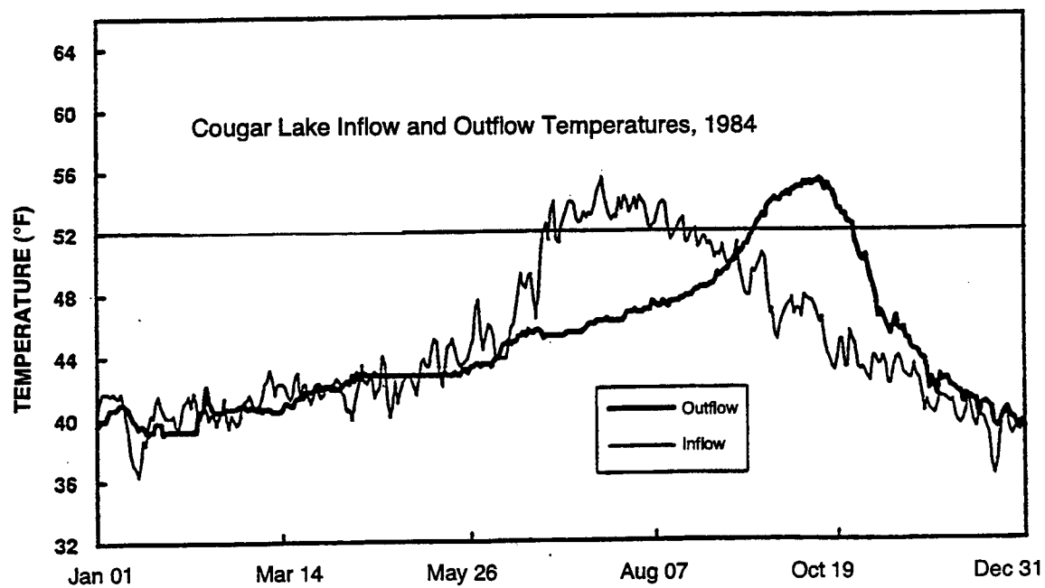
Figure 7. Plots of thermal isopleths and inflow and outflow temperatures for 1984 at Cougar Dam. (Plots reproduced from USACE 1994)
