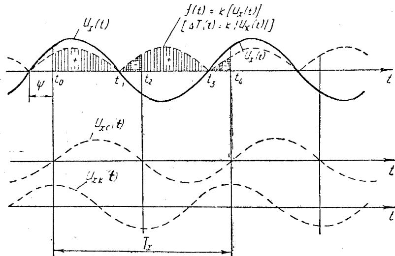
Figure 1. Time Diagram of the Operation of an Integrating Converter in Synchronous Detection Mode
