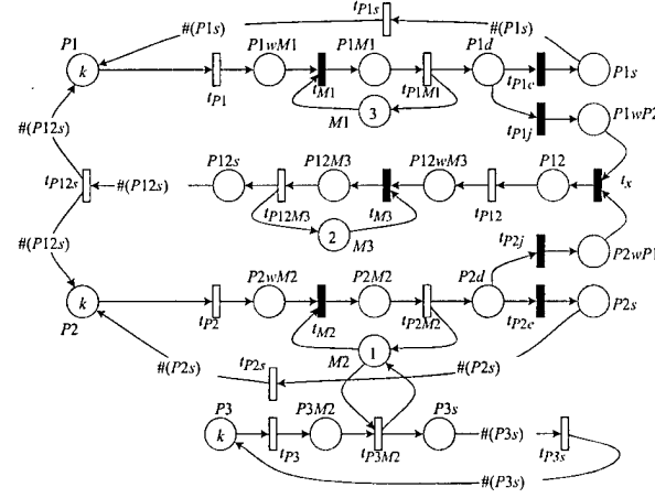
FIG. 6.1. Petri Net Model of a Flexible Manufacturing System. White transitions are timed, black transitions are immediate. Expressions in places denote the number of tokens in the initial marking, labels on places and transitions are used for description, and labels on arcs describe the number of tokens transferred by the firing of the connected transition.
