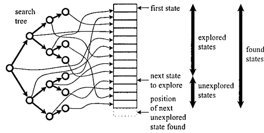
FIG. 2.1. Organization of explored, unexplored, and found states.
