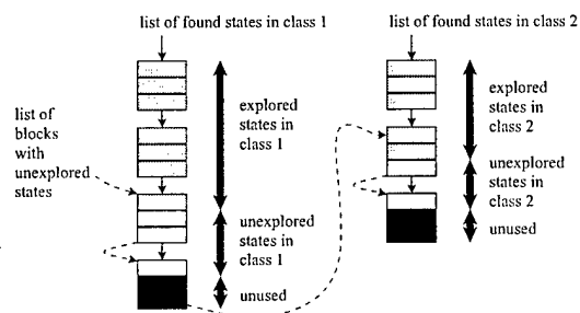
FIG. 3.2. Block-oriented organization of class-grouped states in a given processor, assuming that it is assigned classes 1 and 2.
