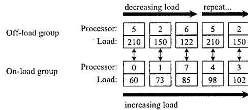
FIG. 4.1. Pairing of source and destination processors
