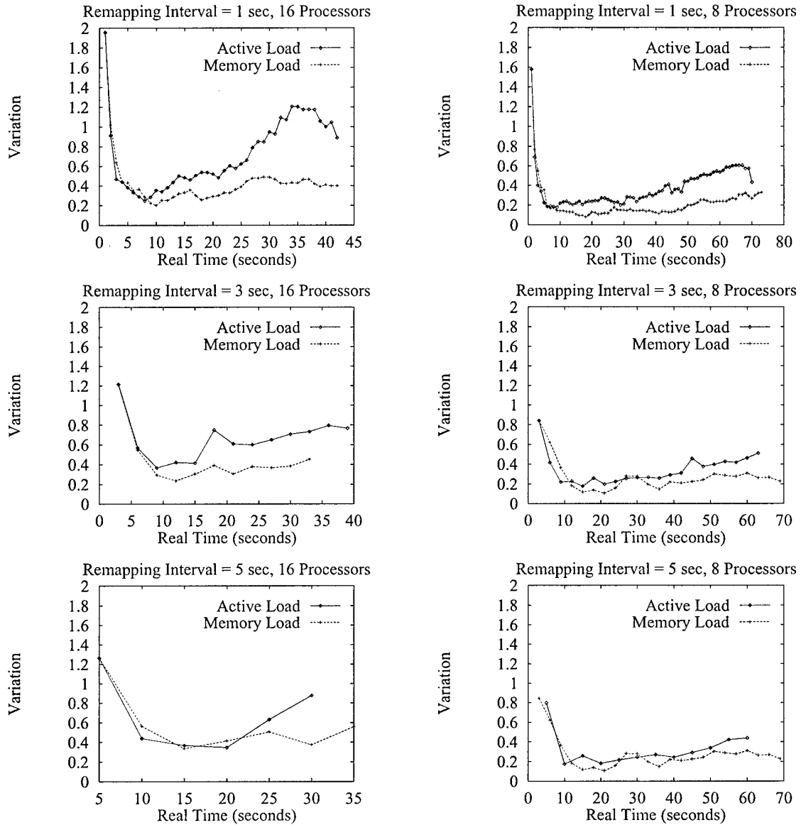
FIG. 6.5. Variation in memory utilization, as a function of time. Variation is measured as average ratio of the difference between maximum and minimum memory usage to average memory usage.
