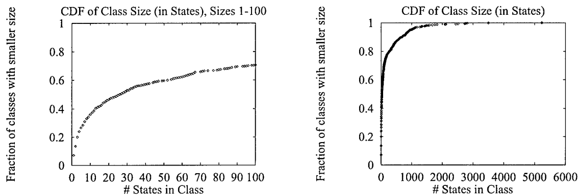
FIG. 6.2. Cumulative distribution function of class size
