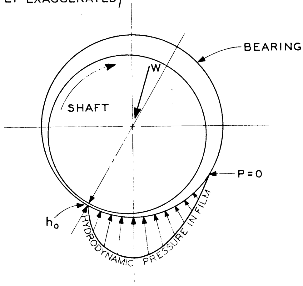
FIGURE 2 HYDROLYNOMIC JOURNAL BEARING
