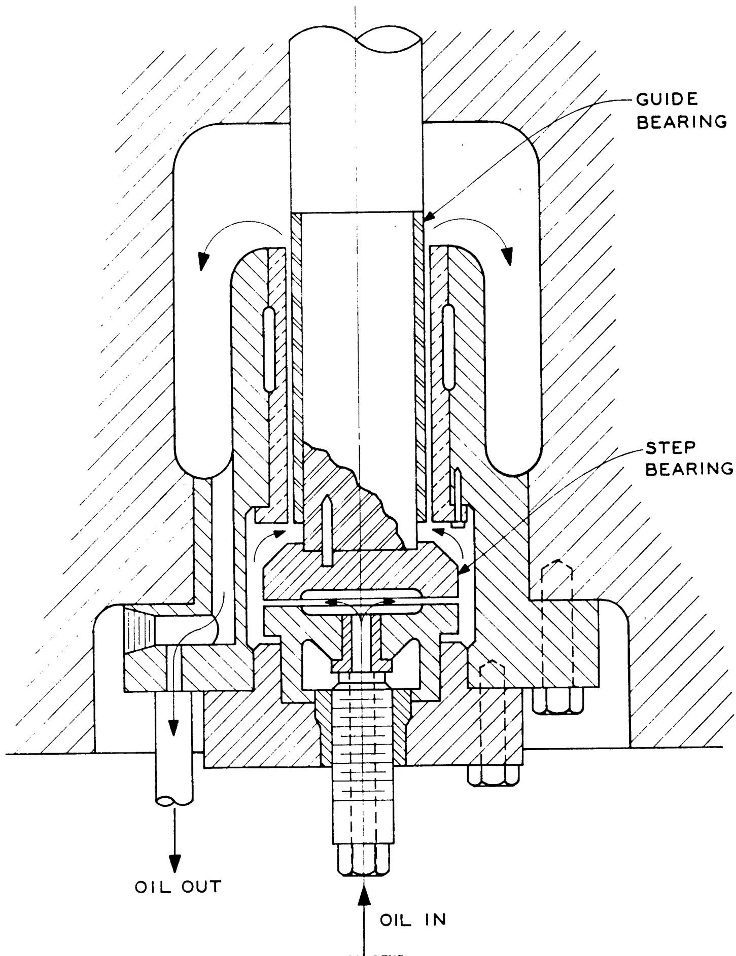
FIGURE 7 STEP THRUST BEARING
