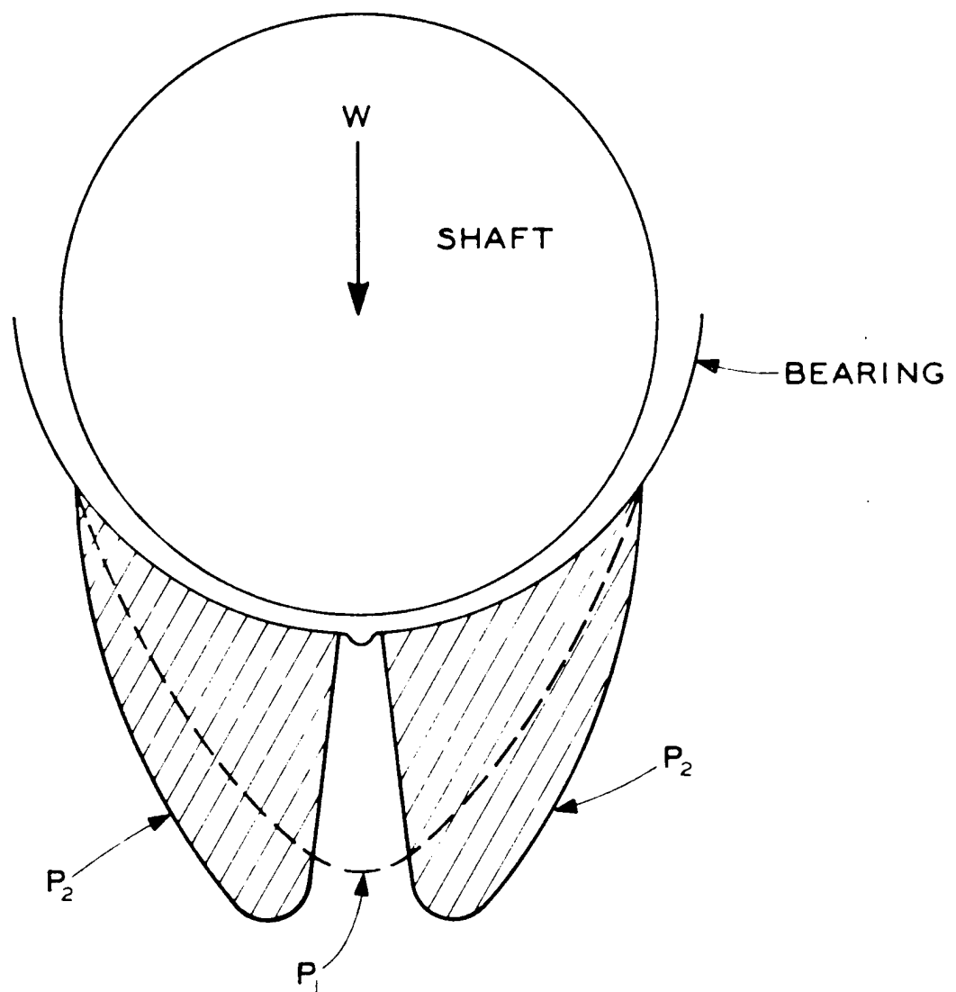
FIGURE 5 GROOVE EFFECTS ON HYDRODYNAMIC PRESSURE
