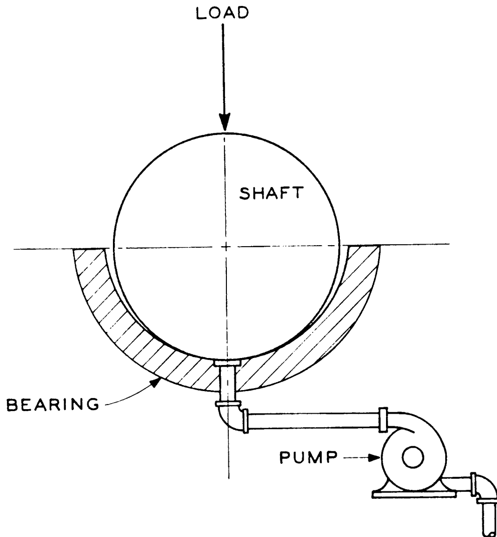
FIGURE 8 OIL LIFT BEARING
