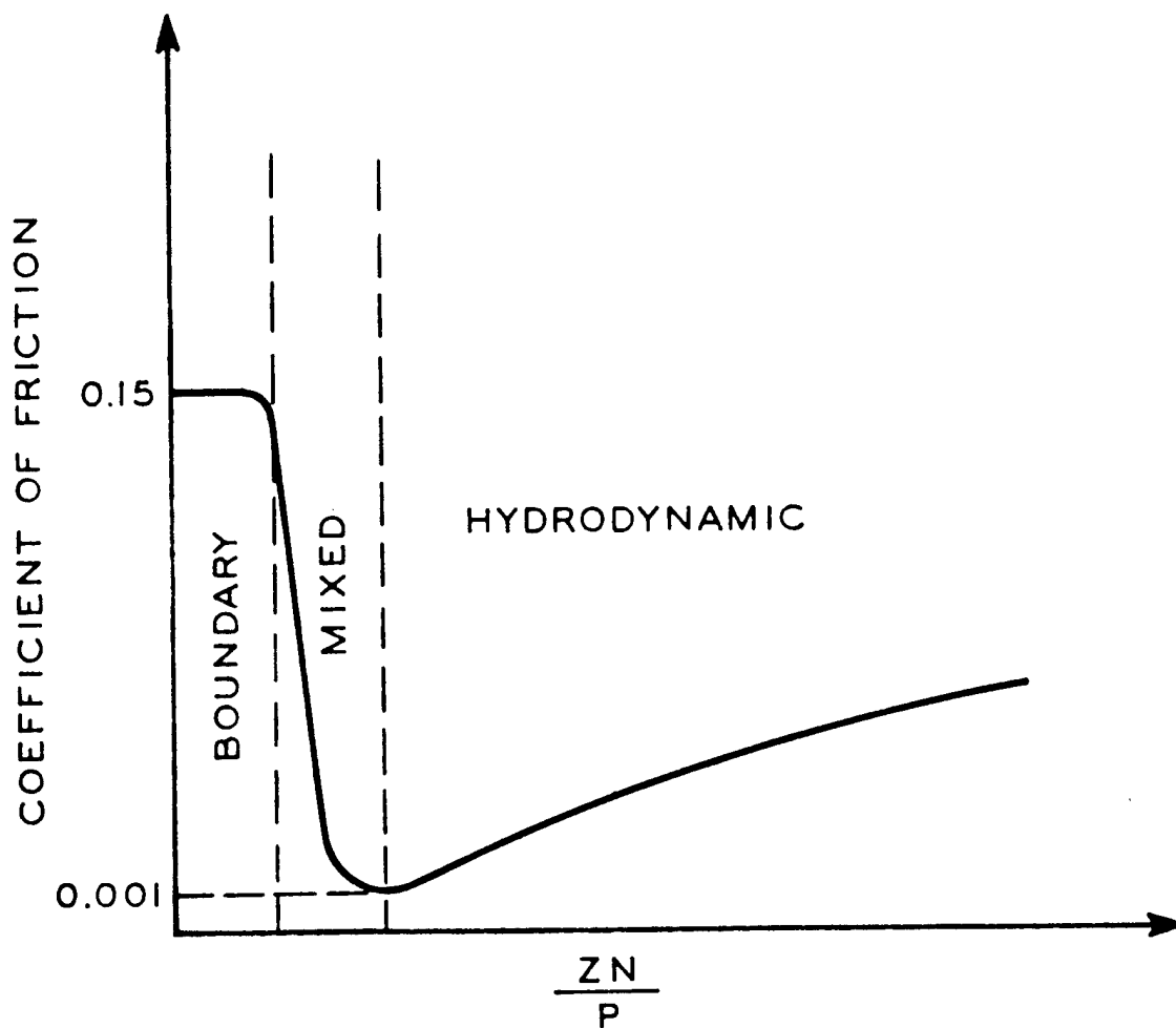
FIGURE 3 FRICTION VERSUS \frac{ZN}{P}
