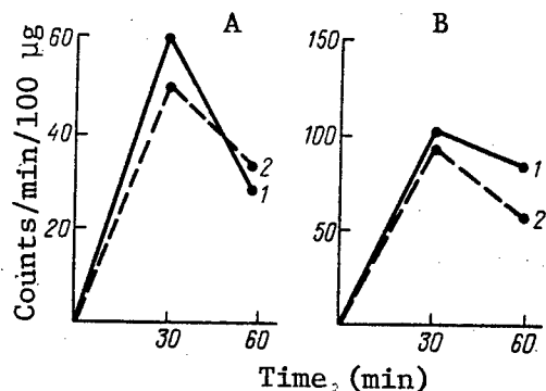
Figure 2. Incorporation of 14 C-glycine in insulin of pancreas slurry from intact (vivarium) and flight rats
