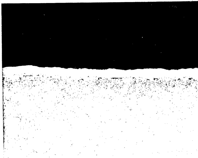
FIGURE 10. PHOTOMICROGRAPH OF VAPOR DEPOSITED CHROMIUM CARBIDE OVERCOATED WITH ALUMINA ON EXTRUSION PARTS
