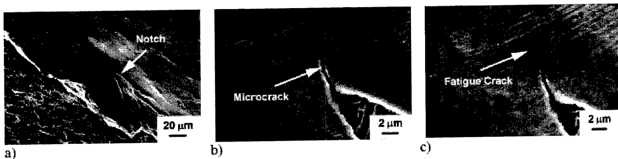
FIGURE 17. Scanning electron micrographs showing the presence of microcracking at crater rim of a FOD indent after the highest velocity (300 m/s) impacts. Micrographs show (a) local notches at crater rim caused by plastic flow of material, (b) microcracks emanating from such notches, and (c) subsequent fatigue-crack growth initiated at such microcracks after 5,000 cycles at \sigma_{\max} = 500 MPa ( R = 0.1 ).
