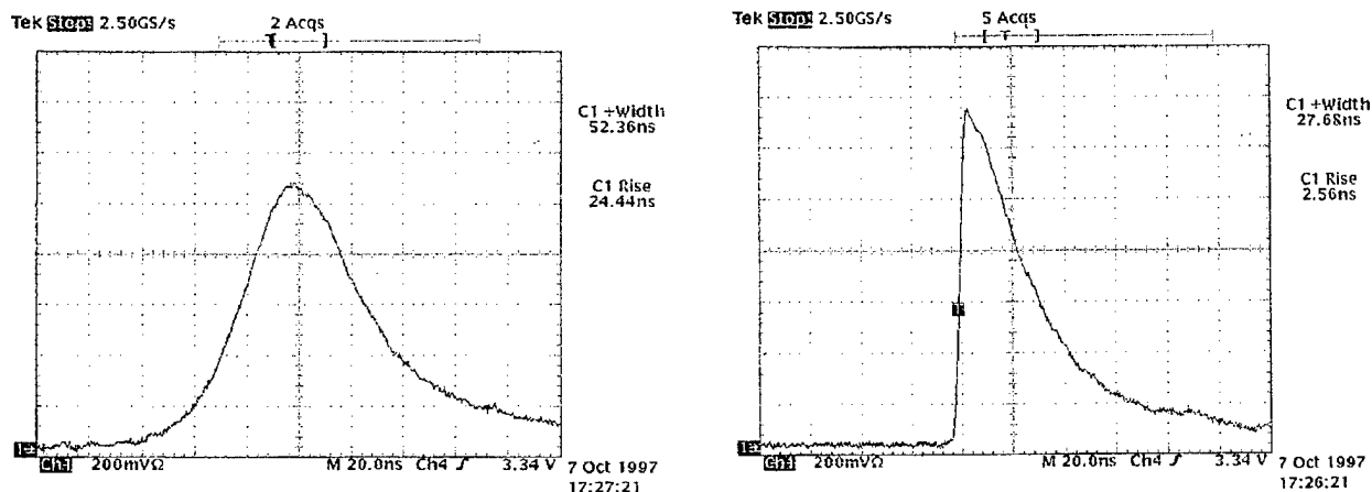
FIGURE 4. Peak Rise Time Before & After Laser System Modifications
