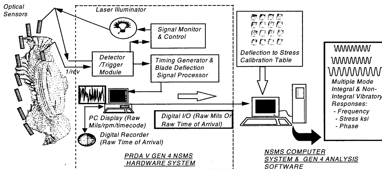
FIGURE 23. Next-Generation NSMS Overview
