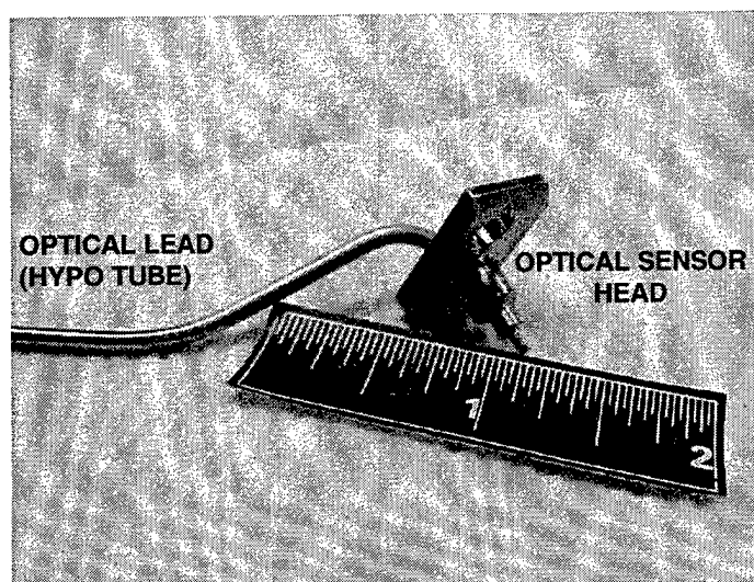
FIGURE 25. F100-220 First-Stage High Compressor NSMS Flight Probe
