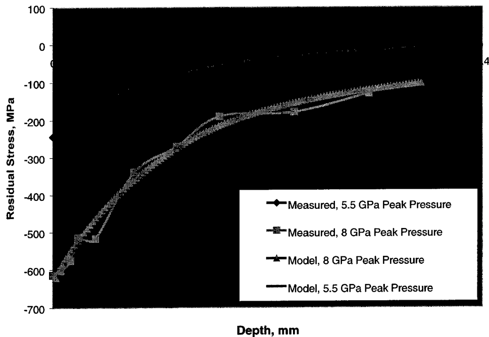
FIGURE 6. Comparison of Modeled and Experimental Residual Stresses for Similar Pressure Conditions
