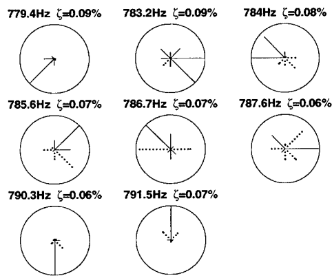
FIGURE 41. Mode Shapes for the Mistuned, Coupled Case
