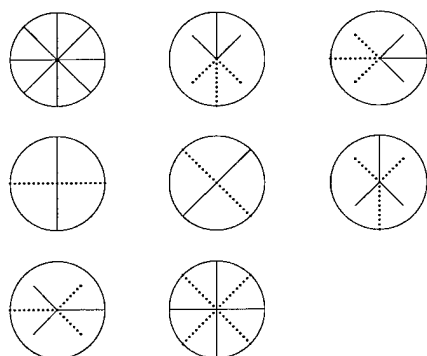
FIGURE 39. Extended Mode Shapes for Eight Blades
