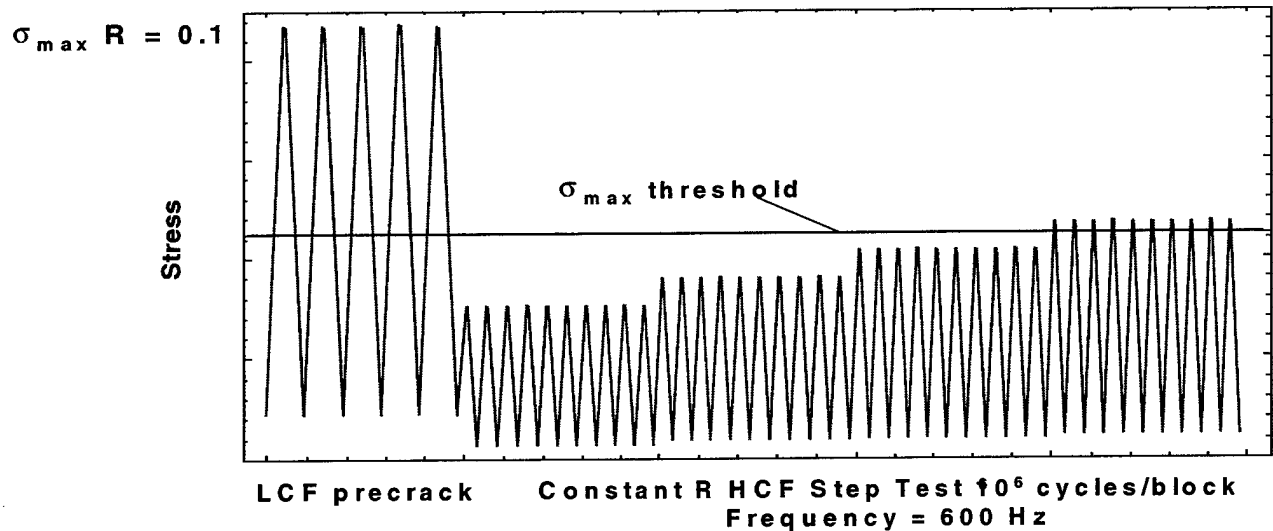
FIGURE 9. Pre-Crack and Step-Test Loading Technique Used to Determine LCF/HCF Thresholds
