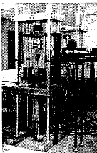
FIGURE 58. Proof of Concept Biaxial Fatigue Fixture
