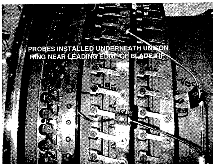
FIGURE 26. F100-220 First-Stage High Compressor NSMS Optical Probe Lead Routing
