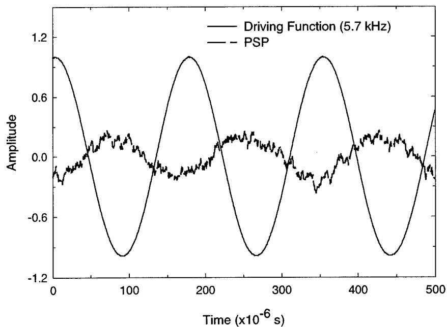
FIGURE 28. PSP Response to a 0.2-psi Pressure Modulation at 5.7 kHz
