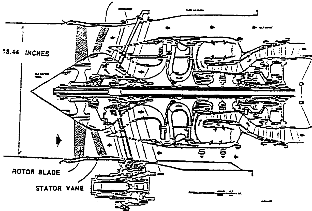
FIGURE 35. Schematic of F109 Engine Showing Location of Pressure-Instrumented Stators
