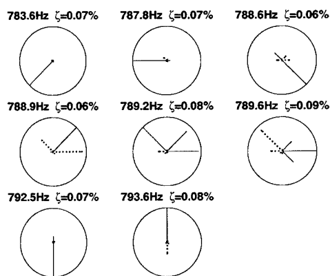
FIGURE 40. Mode Shapes for the Mistuned, Uncoupled Case
