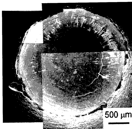
FIGURE 16. Scanning electron micrographs of impact damage sites for a 300 m/s impact velocity, indicating lip formation at crater rim and intense shear band formation emanating at the indent surface.
