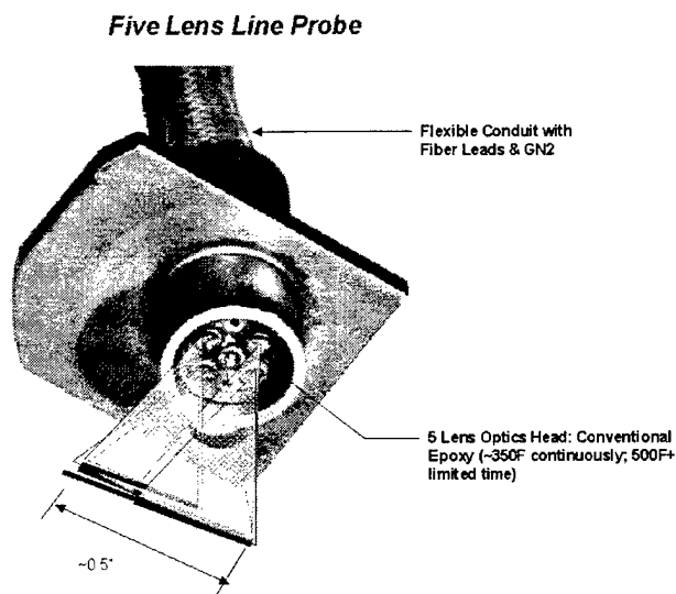
FIGURE 24. Five-Lens Line Probe
