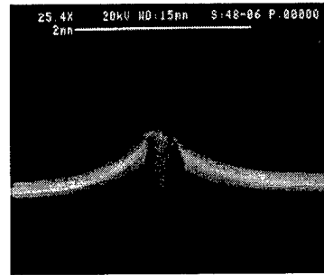
FIGURE 19. Representative FOD from Ballistic and Solenoid Gun Impacts (Sharp Leading Edge Specimens, 30° Impacts, High Damage Levels)
