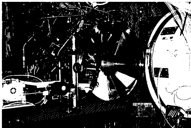
FIGURE 5. PSP Test Setup (ISP – Pink, TSP – White, PSP – Yellow).
