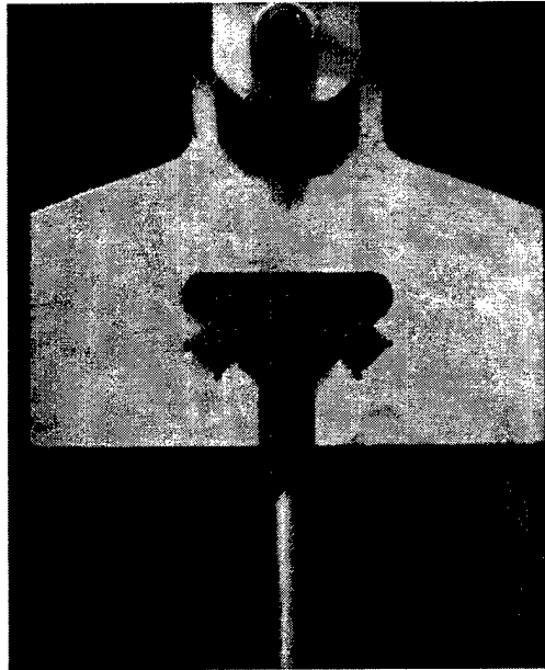
FIGURE 13. New HCF/LCF Fretting Fatigue Test Apparatus
