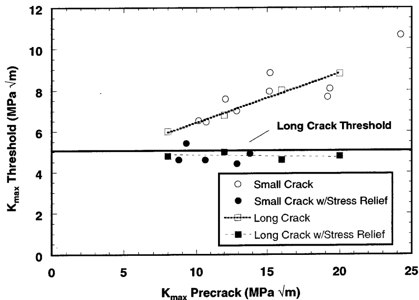
FIGURE 10. LCF/HCF Thresholds for HCF Stress Ratio R=0.1
