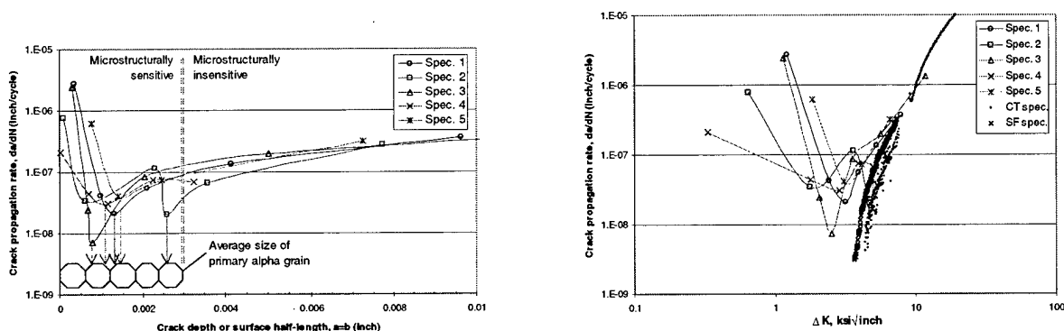
FIGURE 18. Fatigue Crack Propagation Rate of Naturally-Initiated “Small” Cracks as a Function of: (A) Crack Size and (B) Stress Intensity Factor Range.
