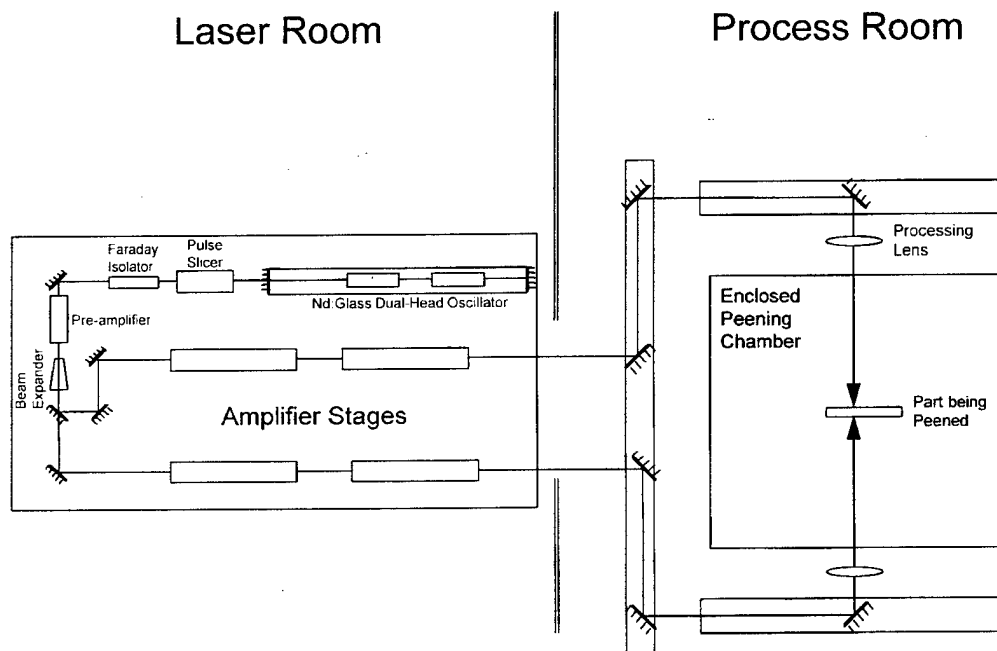
FIGURE 5. Schematic of Laser System Operations
