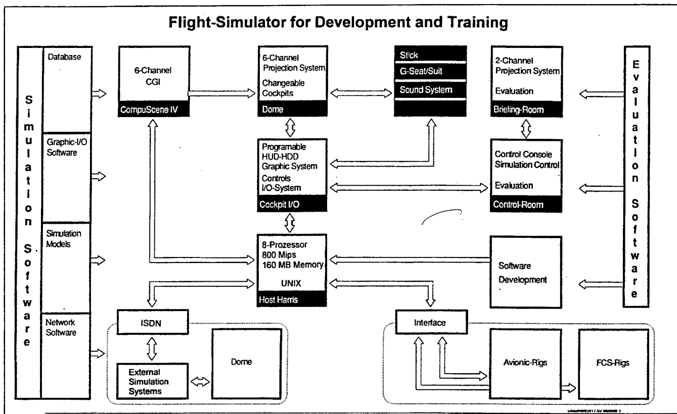
Fig. 2-4 Block diagram of the Dasa Dome Simulation
