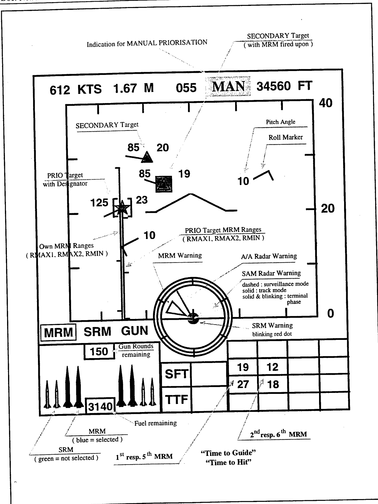
Fig. 3-30 Combat Display Symbology ( MRM selected )
