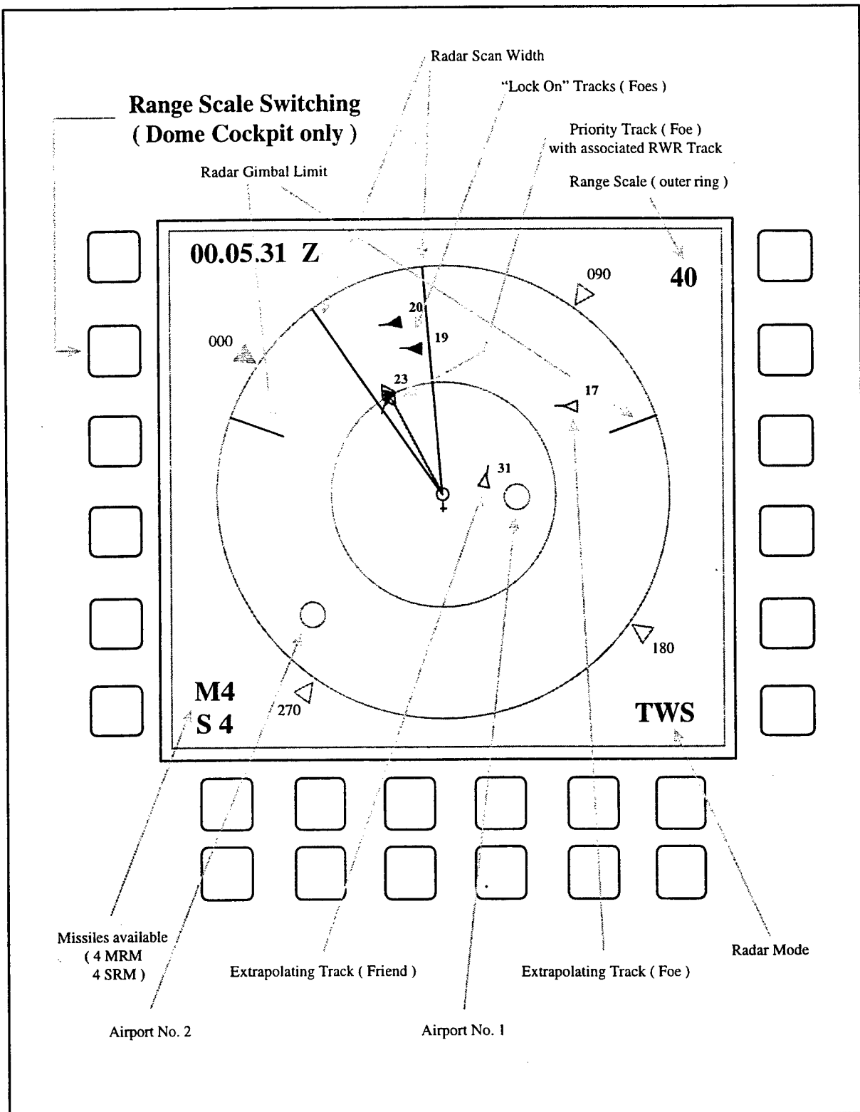
Fig. 3-31 CTI Display Symbology
