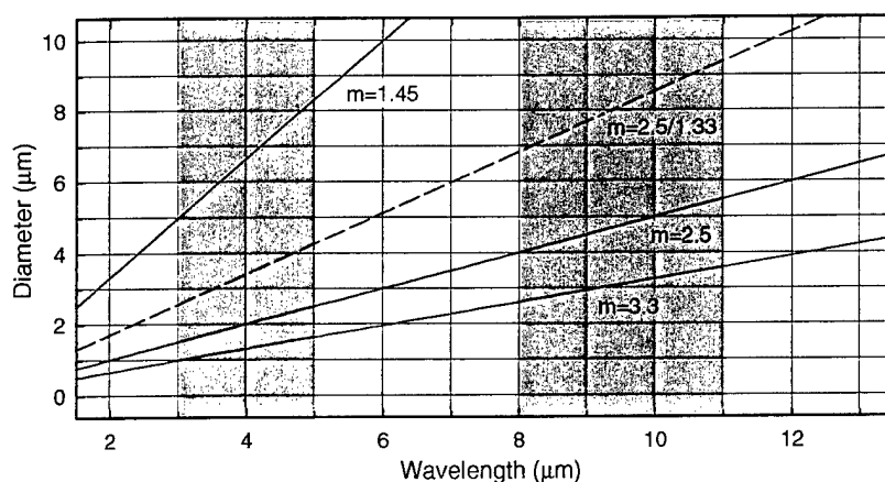
Fig. 3 - Plot of particle diameters that yield maximum extinction as a function of wavelength for several materials based on the approximate solution (Eq. (9)) to the extinction curve. The values of m are close to those for the materials investigated: m = 1.45 , salts; m = 2.5 , silicon carbide, iron oxide, and titanium oxide; m = 3.3 , graphite. The dashed line indicates results for aqueous suspension (in which case the wavelength axis should be taken as \lambda/m_2 , where m_2 is the index of the liquid - 1.33 for water).
