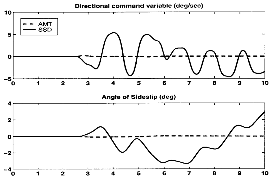
Figure 4.2: Mach 0.35, 5000 ft. Altitude, Zero Dynamics Stability
