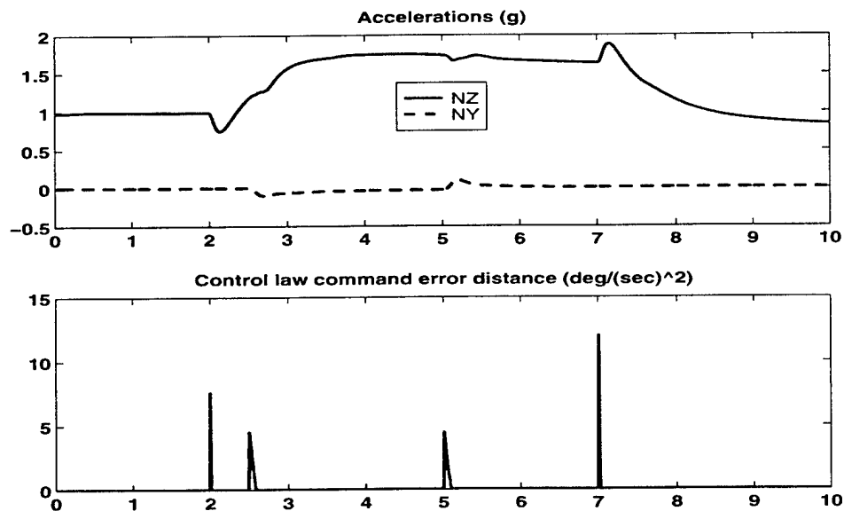
Figure 4.81: Mach 0.35, 5000 ft. Altitude, Min Vec CA Mode
