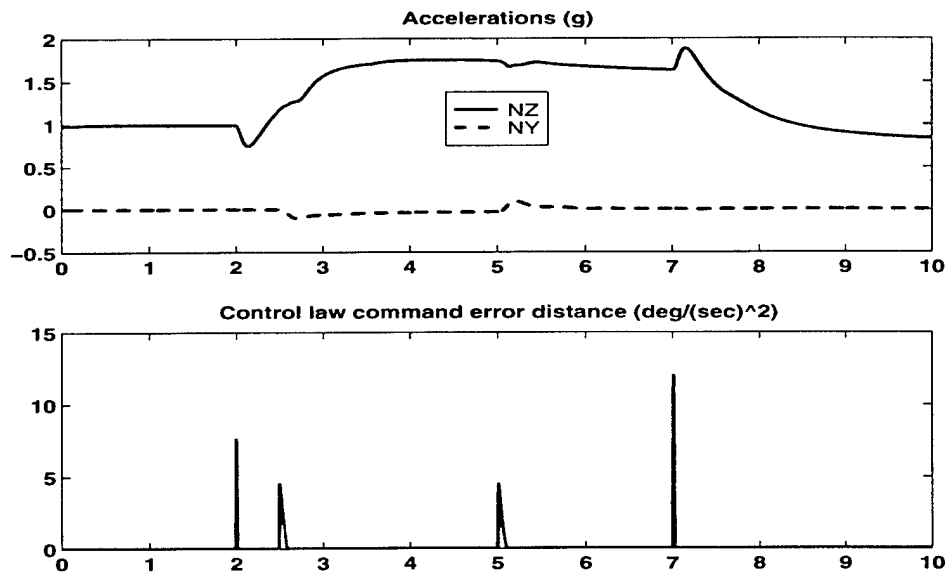
Figure 4.26: Mach 0.35, 5000 ft. Altitude, Min Def CA Mode
