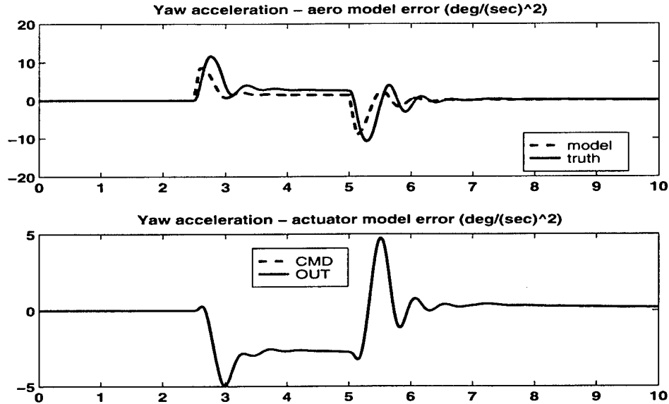
Figure 4.62: Mach 0.35, 5000 ft. Altitude, Min Signature CA Mode
