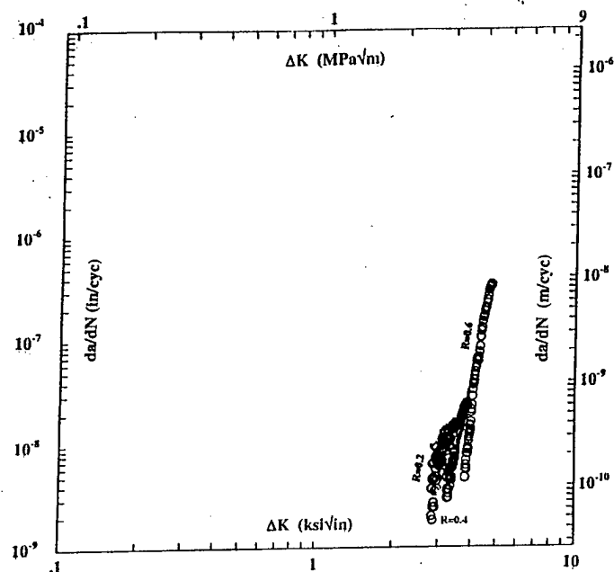
FIG. 4 – Data showing variation of fatigue crack growth rate da/dN with stress intensity Range \Delta K at stress ratios R = 0.2, 0.4, and 0.6 in vacuum.
