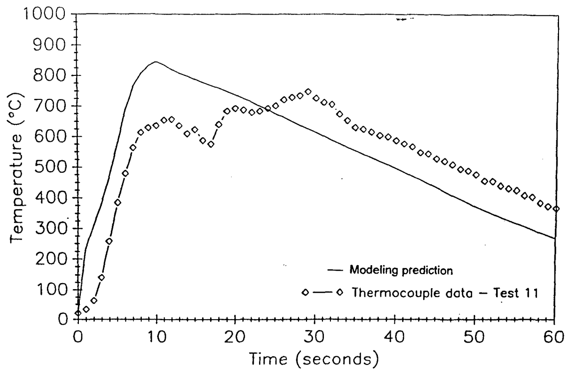
Figure A - 11. Modeling prediction compared to HULVUL data for Test 11, upper layer temperature
