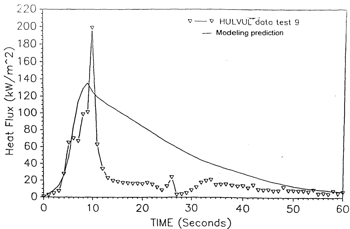
Figure A - 20. Modeling prediction of heat flux at floor level as compared with HULVUL data for Test 9
