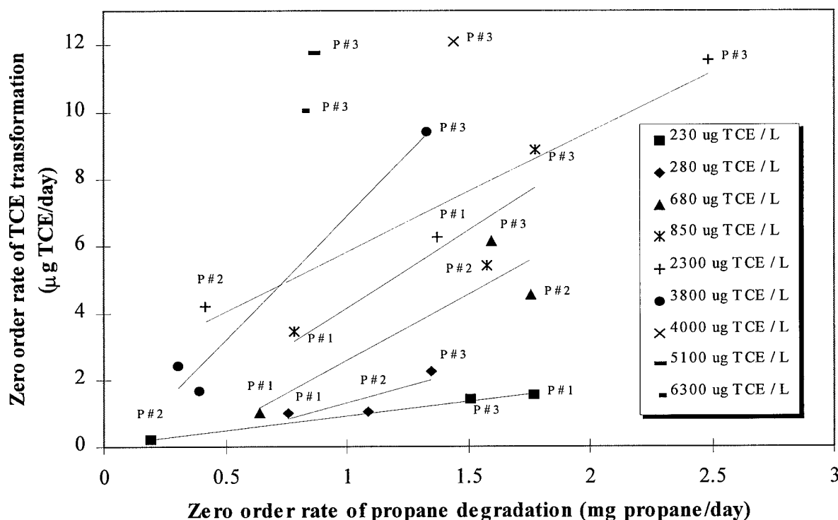
Figure 32. Effects of aqueous TCE concentration on the initial TCE transformation and propane utilization-fits in three propane-utilizing microcosms. Solid lines are the linear regression best-fits at different aqueous TCE concentrations.
