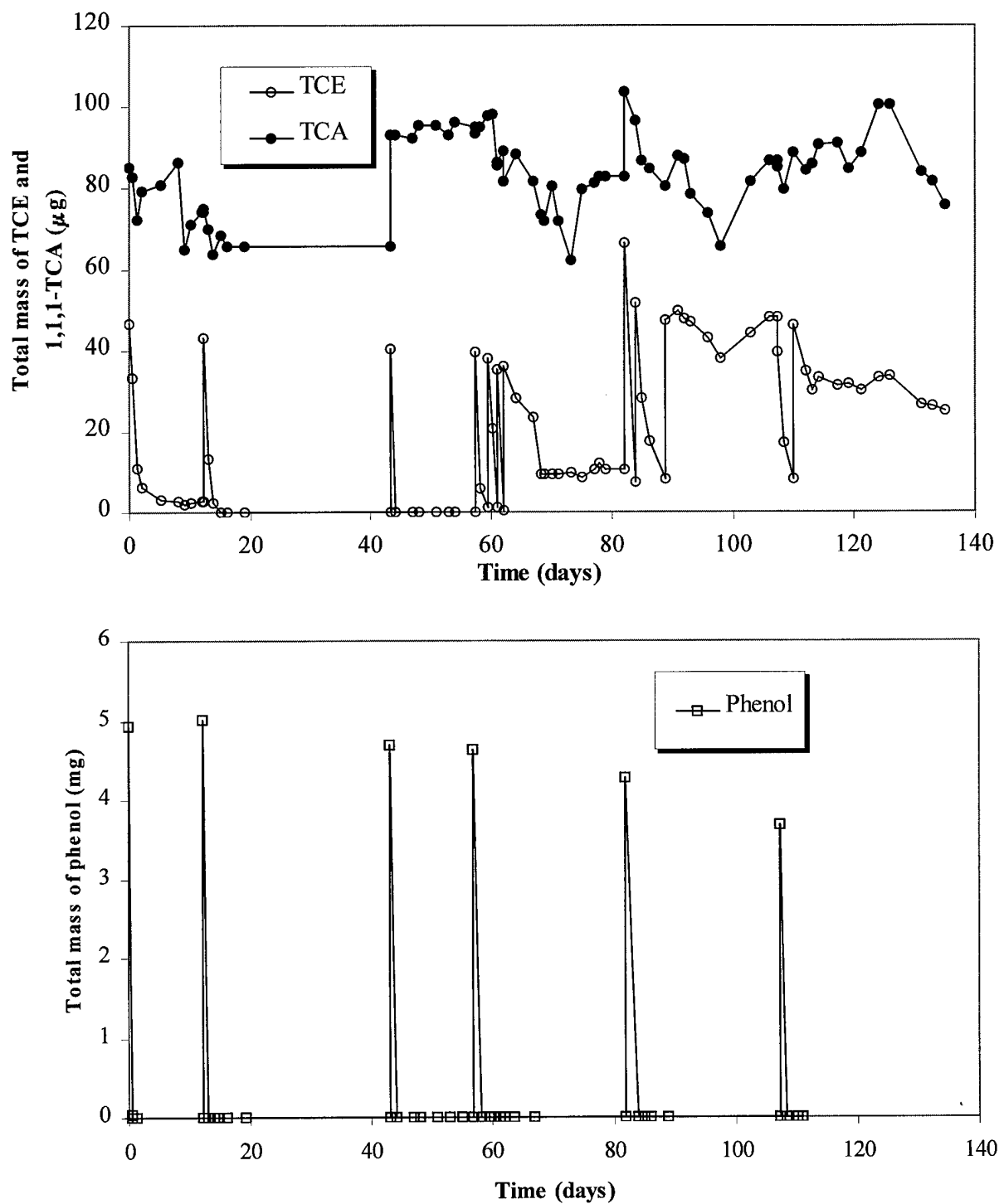
Figure 58. TCE and 1,1,1-TCA transformation in phenol-fed microcosm (Ph#1)
