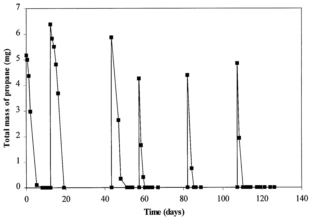
Figure 57. TCE and 1,1,1-TCA transformation in propane-fed microcosm PR#1
